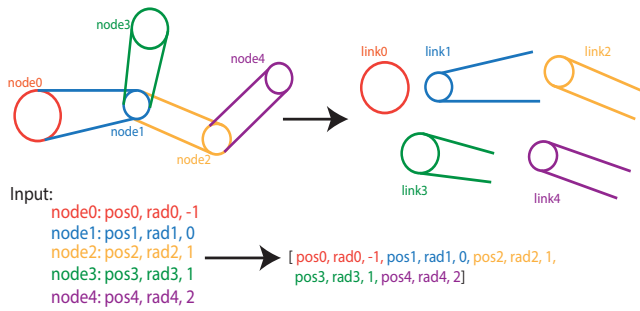
Figure 2: Illustration of the input data structure. We make a list of control points, each with a position, radius, and predecessor index. Each control point and its cylinder or cone stump connection to its predecessor is referred to as a “link”.
