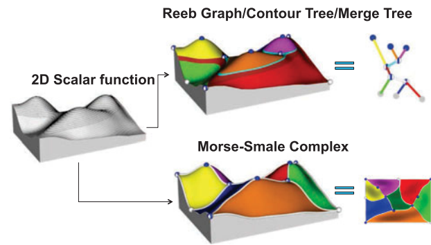
Fig. 3. Contour- and gradient-based topological structure of a 2D scalar function.
