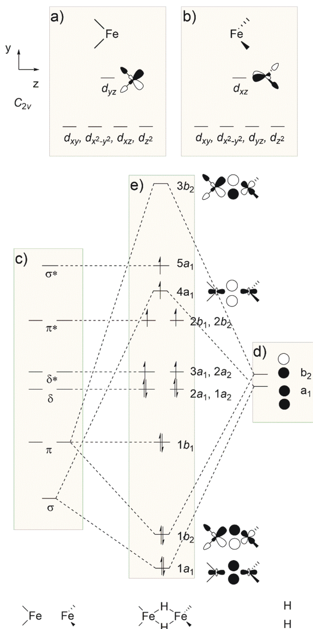
Figure 4. Qualitative MO analysis for [\text{Ph}_2\text{B}(\text{'BuIm})_2\text{FeH}]_2 , assuming C_{2v} symmetry and with the [\text{Fe}_2\text{H}_2]^{2+} core in the yz plane. Fragment orbitals for (a) square planar and (b) tetrahedral \text{L}_2\text{Fe} iron sites, including 3d-4p mixing, used to construct the fragment orbitals of (c) the \text{L}_2\text{Fe}\cdots\text{FeL}_2 fragment. The final MO diagram obtained from mixing this fragment with the 2\text{H} fragment orbitals (d) is shown in panel (e). Additional orbital mixing in this low symmetry environment has been ignored in the interest of clarity.
