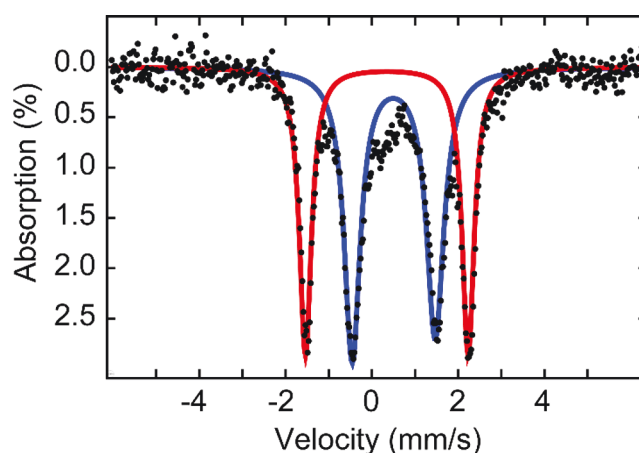
Figure 2. Solid-state Mössbauer spectrum of [\text{Ph}_2\text{B}(\text{'BuIm})_2\text{FeH}]_2 at 80 K. Black circles represent experimental data, while red and blue lines correspond to fits of subspectra I and II, respectively (see text for fit parameters).
