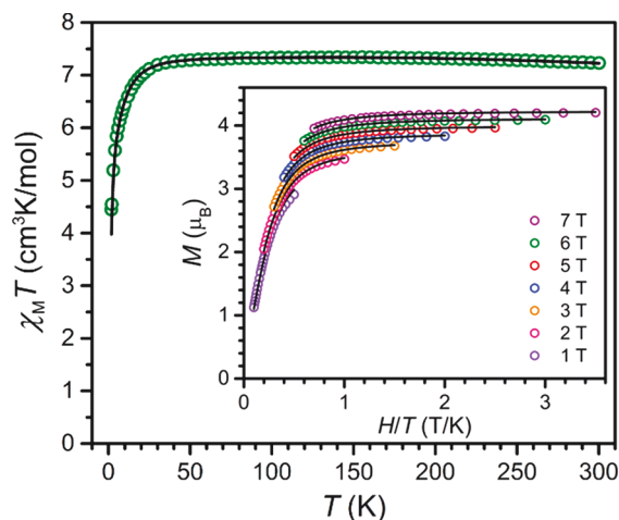
Figure 3. Variable-temperature dc magnetic susceptibility data for [\text{Ph}_2\text{B}(\text{tBuIm})_2\text{FeH}]_2 , collected under an applied field of 5000 Oe, with the black line corresponding to a fit of the data. Inset: Low-temperature magnetization data for [\text{Ph}_2\text{B}(\text{tBuIm})_2\text{FeH}]_2 , collected at selected fields in the temperature range 2–10 K, with the black lines corresponding to a fit of the data (see text for all fit parameters).
