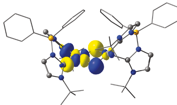
Figure 5. Unrestricted natural orbital representation of the DFT-computed LUMO of [\text{Ph}_2\text{B}(\text{'BuIm})_2\text{FeH}]_2 with orbital isodensity at 0.05.
