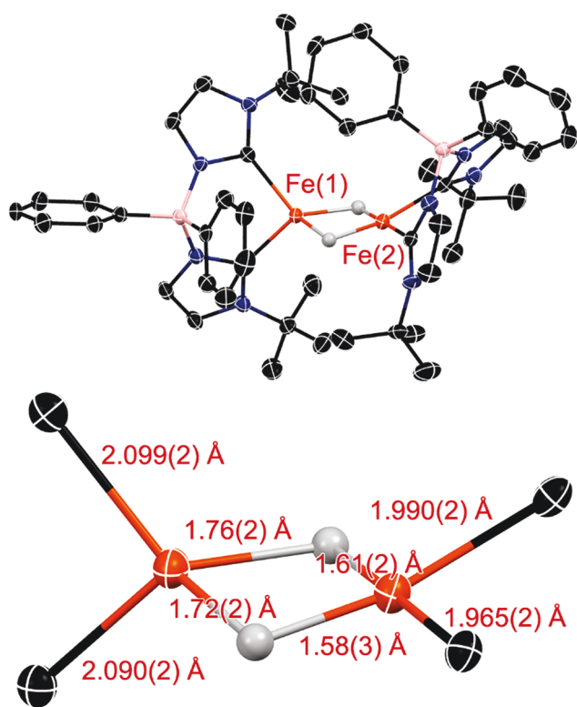
Figure 1. Top: X-ray crystal structure of [\text{Ph}_2\text{B}(\text{'BuIm})_2\text{FeH}]_2 . Thermal ellipsoids shown at 50% probability; peripheral hydrogen atoms omitted for clarity. Bottom: Core structure of the molecule, with selected bond lengths. Black, white, blue, pink, and orange ellipsoids represent carbon, hydrogen, nitrogen, boron, and iron atoms, respectively.
