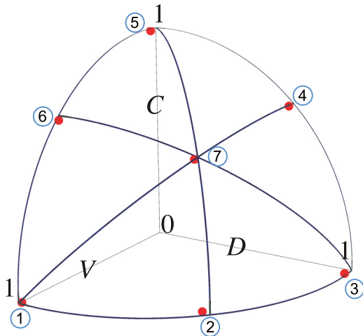
FIG. 3. An octant is shown of the VDC sphere defined by the QVE duality identity V^2 + D^2 + C^2 = 1 . Our experiments subject a generic single-photon pure state to a variety of different two-beam interference experiments. These yield a wide range of V and D values. The observed values of V^2 + D^2 vary from 0 to 1, but in all cases remain on the surface of the VDC sphere, consistent with Eq. (2).
