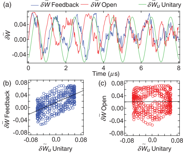
FIG. 4. Work along trajectories with and without feedback. (a) the instantaneous work \delta\tilde{W} along a single trajectory in the presence of feedback (blue) and the open loop configuration (no feedback) (red) is compared to the calculated instantaneous work expected for pure unitary evolution (green). (b),(c) The correlation between the instantaneous work \delta\tilde{W} and the work for a unitary evolution along a quantum trajectory. The linear regression fit (black lines) show correlation (slope 0.44, estimated error 0.03) when the feedback loop is employed, and no correlation in the open loop configuration (slope 0.007, estimated error 0.04).
