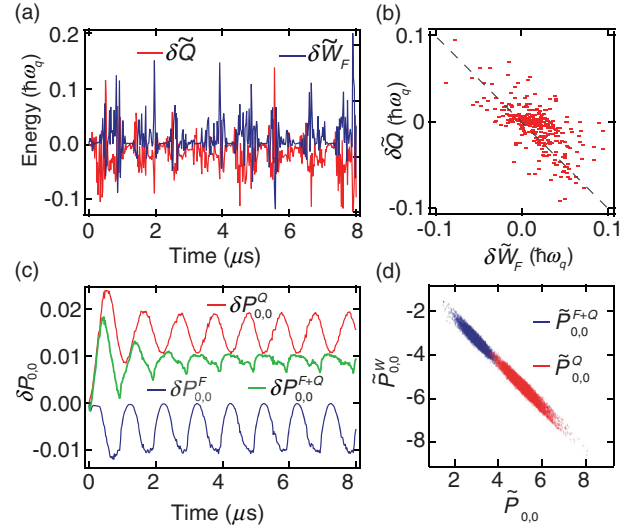
FIG. 3. Quantum feedback loop. (a) Instantaneous heat and feedback work along a single trajectory. The feedback work has been time shifted by 20 ns to account for the time delay in the feedback circuit. The anticorrelation ( r = -0.68 ) of heat and feedback work is evident in the scatter plot (b). (c) Average of the instantaneous contribution of heat and feedback to the transition probability for 10^4 experimental iterations. (d), Parametric plot of \tilde{P}_{0,0}^W versus \tilde{P}_{0,0}^Q (red) and \tilde{P}_{0,0}^{F+Q} (blue) showing how the feedback cancels the heat, narrowing, and shifting the distribution toward zero for \tau = 6 \mu\text{s} .
