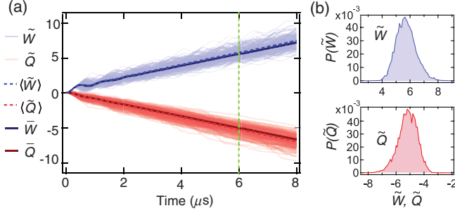
FIG. 2. Comparison of stochastic and average heat and work quantities. (a) Individual heat and work trajectories, \tilde{Q} , and \tilde{W} , are displayed as transparent red and blue traces. The mean of these individual trajectories, \langle \tilde{Q} \rangle , and \langle \tilde{W} \rangle , are displayed as dashed lines which are in good agreement with the mean values from the master equation, \bar{Q} and \bar{W} , Eq. (3), solid lines. (b) Distributions of \tilde{Q} and \tilde{W} at evolution time \tau = 6 \mu\text{s} .
