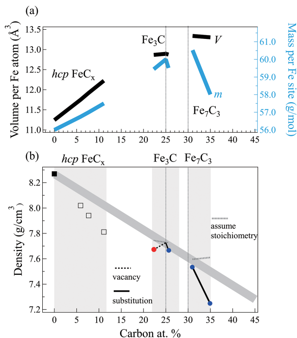
FIGURE 7. The (a) volume and mass per iron atom, and (b) density of \text{FeC}_x , \text{Fe}_3\text{C} , and \text{Fe}_7\text{C}_3 as a function of carbon content. In b, the gray line is drawn through pure hcp \text{ Fe} and stoichiometric \text{Fe}_3\text{C} . The dotted lines represent densities calculated by assuming stoichiometric composition. The dashed and solid lines correspond to the densities calculated by applying the carbon vacancy or C-Fe substitution mechanism, respectively. (Color online.)
