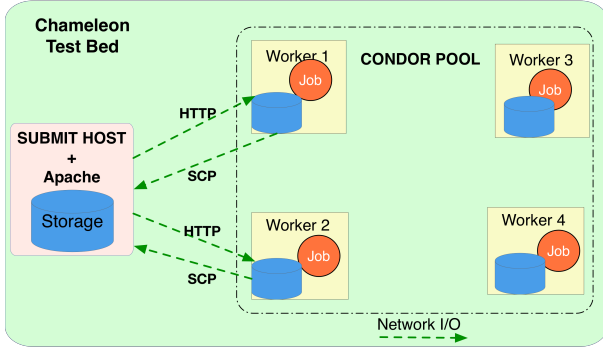
Fig. 2. Non Shared Filesystem Setup
