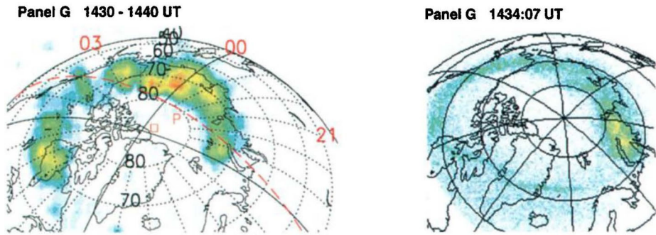
Fig. 13 Example of a diffuse morning side spot emission in X-rays (left) but nothing is seen in UV emissions (right). Adapted from Østgaard et al. (1999)
