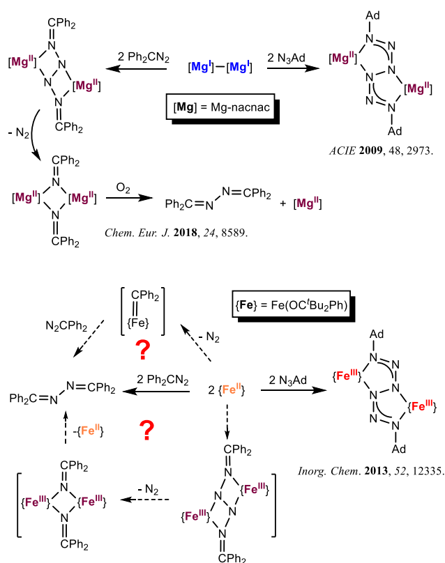
Scheme 1. Top: \text{Mg}^{\text{I}} -nacnac-promoted reductive coupling reactions of an organoazide (right) and diphenyldiazoalkane (left). Bottom: \text{Fe}(\text{OR})_2 -promoted reductive coupling of \text{AdN}_3 (right) and possible (two-electron and one-electron) mechanisms for the formation of benzophenone azine (left).
