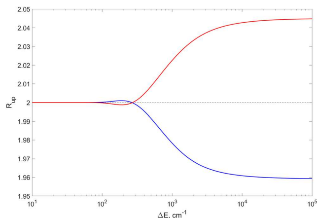
FIG. 6. Ratio of the average number of states in asymmetric and symmetric ozone molecules, as defined by Eq. (1). Blue and red curves correspond to singly and doubly substituted ozone. The horizontal axis gives the averaging energy window size, \Delta E , which in this case is analogous to the thermal energy in the vibrational partition function. The statistical value of two is indicated by the dashed line. The deviations of computed data from this reference are obvious in a broad range of energies. Asymptotically they reach roughly \pm 0.05 .
