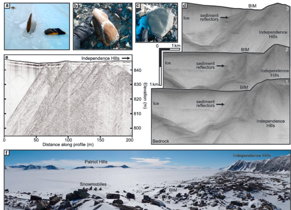
Figure 2. Characterization of Independence Hills Blue Ice Moraine. (a) Sediment emerging from blue ice in Horseshoe Valley. (b) Sediment clast with subrounded shape and straight, parallel striations. (c) Sediment clast with subangular shape and multiple striations, in a variety of orientations. (d) Airborne RES transects across a valley glacier and Independence Hills (shown in photograph f) reveal englacial reflectors which extend from the ice/bed interface to Blue Ice Moraine (BIM) deposits in the lee of Independence Hills. (e) Hyperbolic reflectors in an IPR transect (collected across the BIM sequence at the base of Independence Hills) reveal seven linear features beneath the sediment-strewn surface (shown in photograph f).
