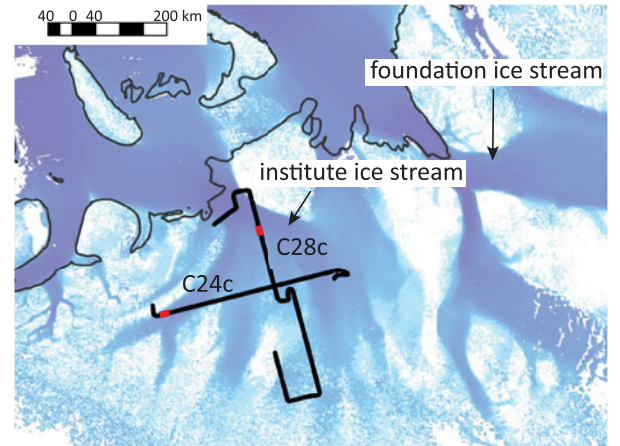
Fig. 6. Radar lines from the BAS-IMAFI survey at Institute Ice Stream. Red segments denote the portions of data analyzed in Figure 7.
