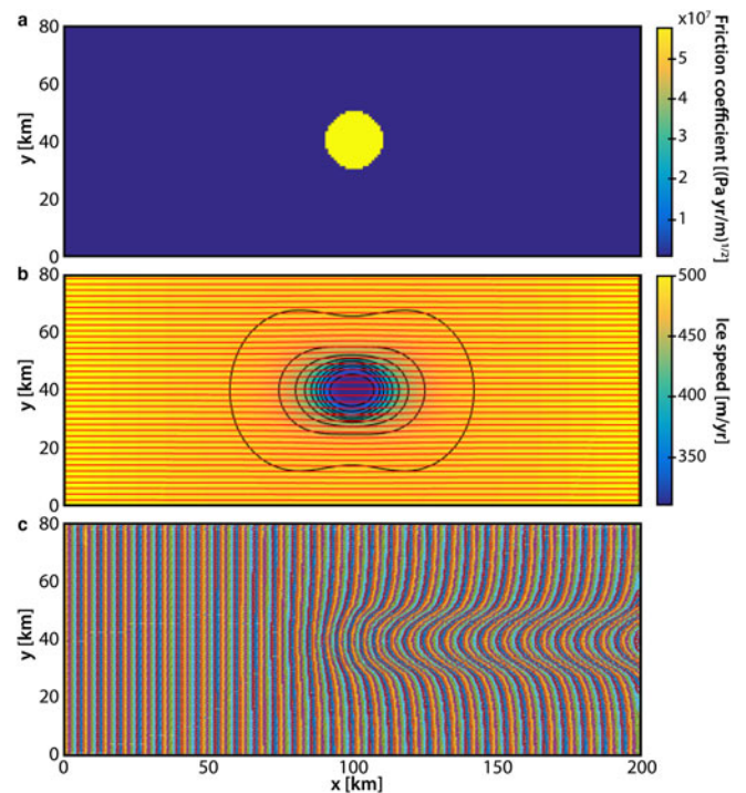
Fig. 4. Simulation of flow over an idealized sticky spot. (a) Uniform basal friction coefficient across the domain, with a centered, abrupt, circular sticky spot. (b) Flow field computed by ISSM, colored by ice speed, and showing streamlines (red). The streamlines do not noticeably deviate from parallel to driving stress. (c) Particles introduced to the flow at x=0 , colored by their introduction time, and advected through the steady-state flow field. There is a distinct rotation and wrapping of the advected particles across the sticky spot, which matches the interpretation of the advected radargrams.
