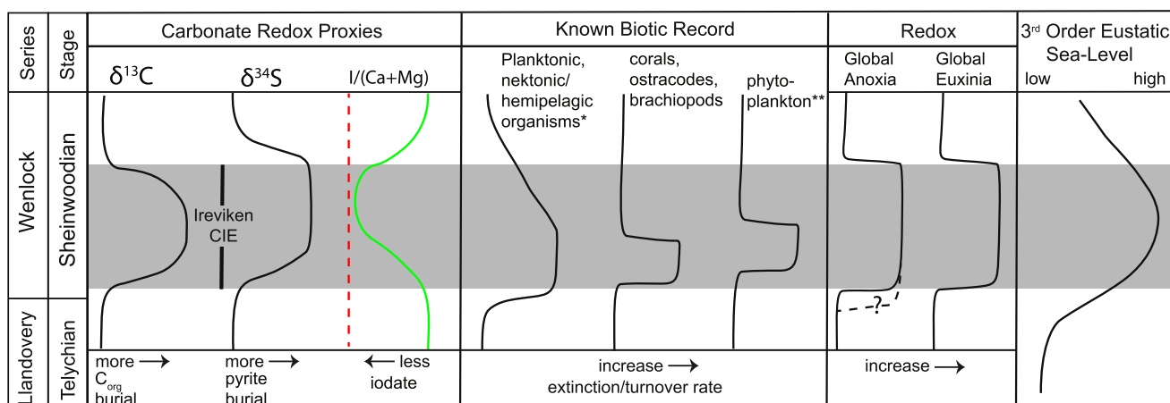
Fig. 5. Generalized stratigraphic changes of carbon and sulfur isotopes ( \delta^{13}\text{C}_{\text{carb}} from Cramer et al., 2010; \delta^{34}\text{S}_{\text{CAS}} from this study) and \text{I}/(\text{Ca}+\text{Mg}) ratios (this study: red, Nevada and green, Tennessee), redox conditions (from this study), and biotic turnover/extinction rates (Jeppsson, 1997; Melchin et al., 1998; Munnecke et al., 2003; Calner, 2008; Cooper et al., 2014) during the Ireviken CIE. *Note that this curve represents the generalized extinction patterns for conodonts and graptolites relative to \delta^{13}\text{C}_{\text{carb}} (e.g., Cramer et al., 2010). **Note that this generalized curve represents acritarch (organic-walled phytoplankton) extinctions of which the majority occurred notably after the other marine extinctions took place (e.g., Calner, 2008). The 3rd order eustatic sea-level curve is modified from Cramer and Saltzman (2007).
