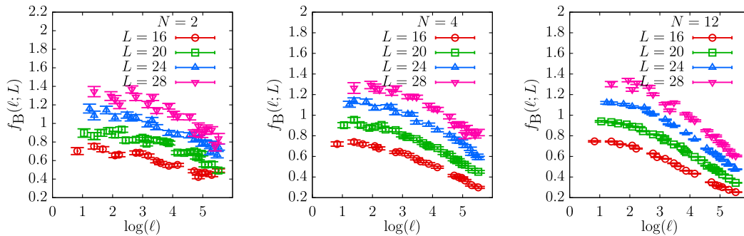
FIG. 2. The bare free energy per fermion degree of freedom, f_B = \mathcal{F}_B/N , of the lattice monopole-antimonopole background field insertion is shown as a function of the physical extent of the box \ell . The three panels from left to right correspond to N = 2, 4 and 12 , respectively. The different colored symbols correspond to different L specified in the key.
