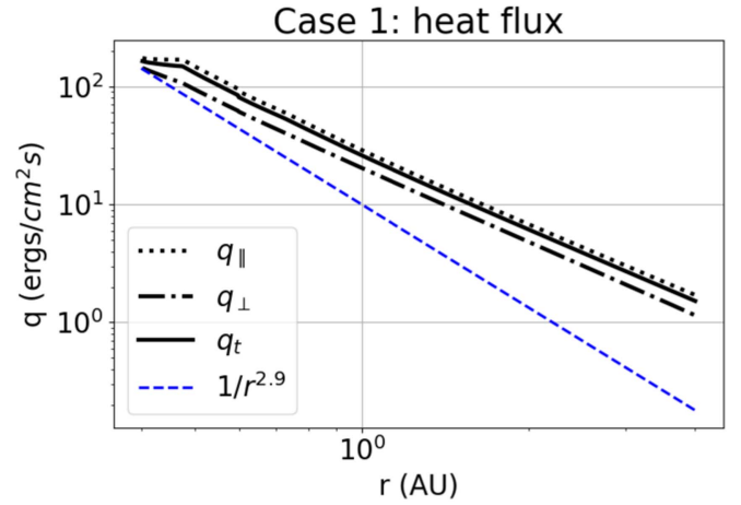
Figure 16. Radial variation of the total q_t , parallel q_{||} , and perpendicular q_{\perp} heat fluxes from about 0.4 to 4 au. The blue dashed line shows q \propto r^{-2.9} , which is obtained from Ulysses observations by Scime et al. (2001).
