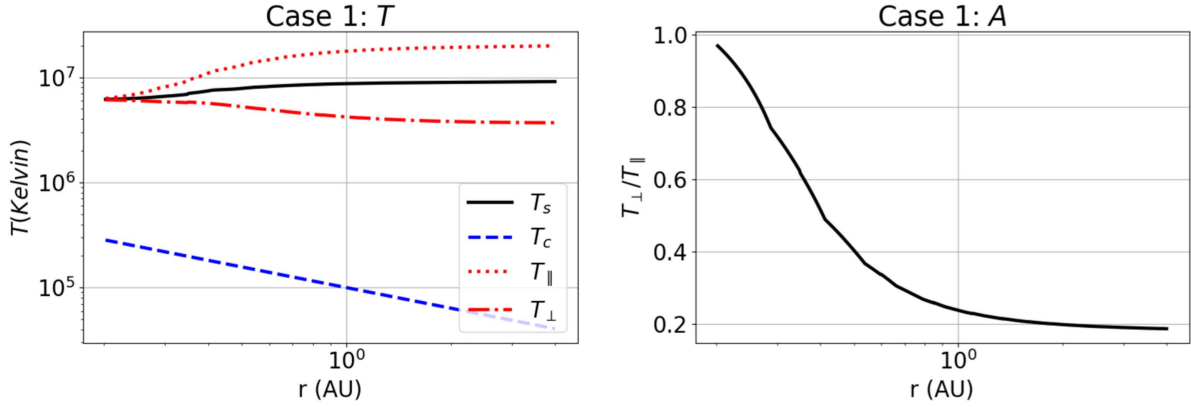
Figure 15. Left: electron temperature vs. distance. The black solid line T_s , red dotted line T_{||} , and red dashed–dotted line T_{\perp} are derived from the suprathermal electron VDF by Equation (33), while the blue dashed line T_c is the temperature of the background Maxwellian core given by Equation (9). Right: radial variation of the temperature anisotropy A = T_{\perp}/T_{||} .
