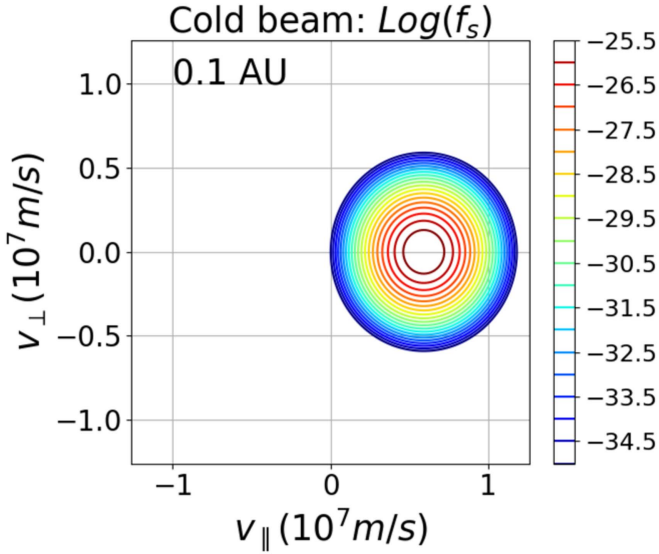
Figure 5. Contour levels of the injected cold beam at the left boundary r_L = 0.1 au.
