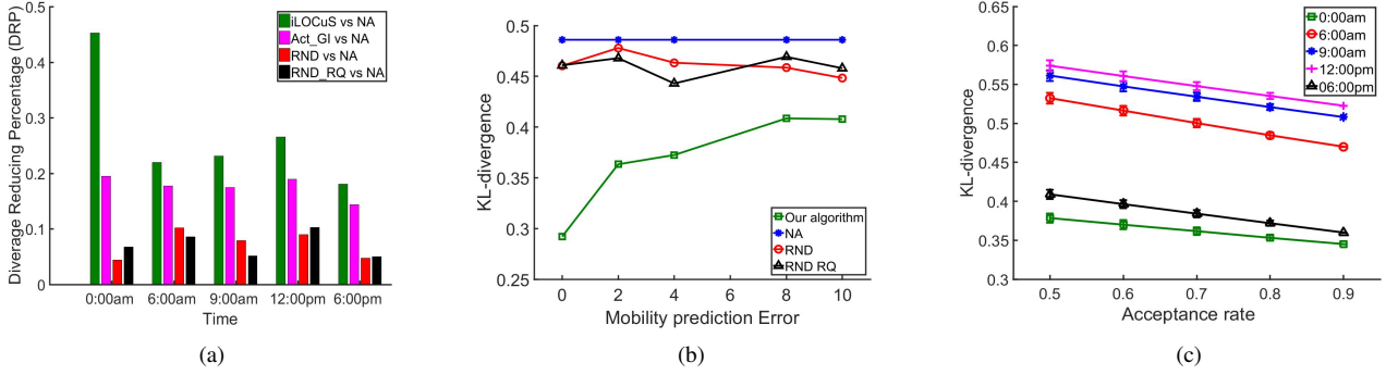
Fig. 11: This figure shows the influence of the incentive design, mobility prediction accuracy, and acceptance rates on the performance of the algorithms. (a) shows the DRP of the KL-divergence by using different incentives and different incentivizing algorithms under Ob_dist_1 at the different time. (b) shows the average KL-divergence changes with different mobility prediction bias at 0:00 am. (c) shows the KL-divergence under different acceptance rates at the different time in one of our experiments.
