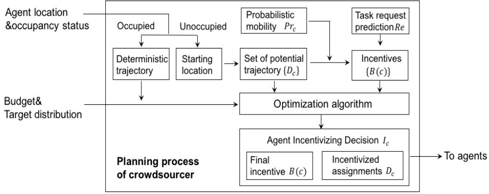
Fig. 3: The flowchart of crowdsourcer's planning process, which is part of the system described in Figure 2.
