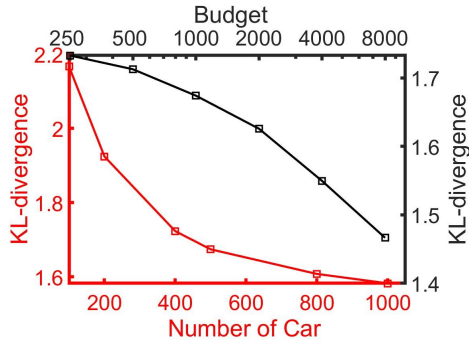
Fig. 10: This figure shows that under Ob_dist_2 , how the KL-divergence of iLOCuS changes with number of cars and budget, respectively. The red line and axes represent the changing of KL-divergence with number of cars. The black line and axes show the changing of KL-divergence with budget.
