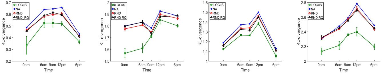
(a) Ob_dist_1 : Uniform distribution over the temporal and spatial domains (b) Ob_dist_2 : Gaussian distribution over the spatial domain (c) Ob_dist_3 : Gaussian mixture distribution over the spatial domain (d) Ob_dist_4 : Gaussian distribution over space and peak changes with time
