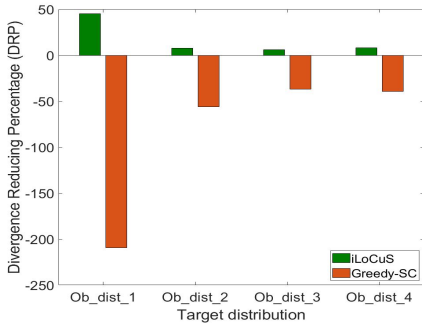
Fig. 7: This figure shows the DRP of iLOCuS and baseline method Greedy-SC. It can be found that since Greedy-SC is designed for a different objective function, using Greedy-SC to incentivize vehicle agents will increase the dissimilarity between the collected data distribution and target distribution compared to not incentivizing any vehicle agents.
