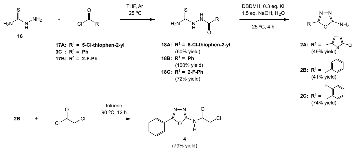
Scheme 1. Syntheses of 1,3,4-oxadiazoles 2A – 2C and 4
