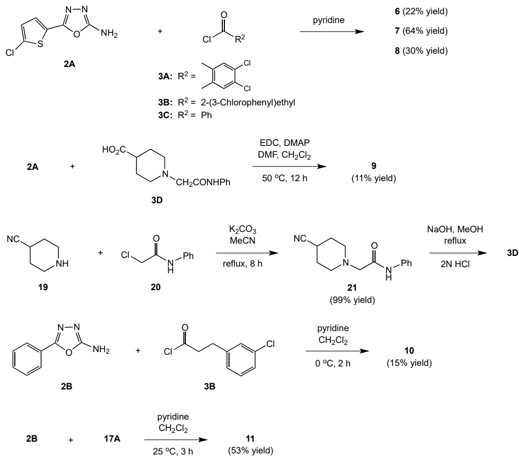
Scheme 2. Syntheses of 1,3,4-oxadiazoles 6 – 11
