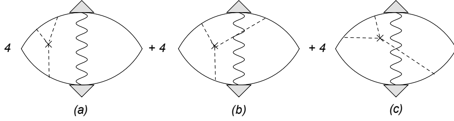
Figure 1: Diagrams for the Maki-Thompson corrections to the AHE in the skew-scattering mechanism. The wavy line represents pair-propagator Eq. (2.5). The shaded triangles stand for the impurity ladder vertex function Eq. (2.3). The dashed lines represent scattering by an impurity, marked by a cross, with the corresponding potential from Eq. (2.7). A factor of four near each diagram represents the total number of equivalent ways to arrange for impurity lines between Green's function per Eq. (2.1) depicted by solid lines.
