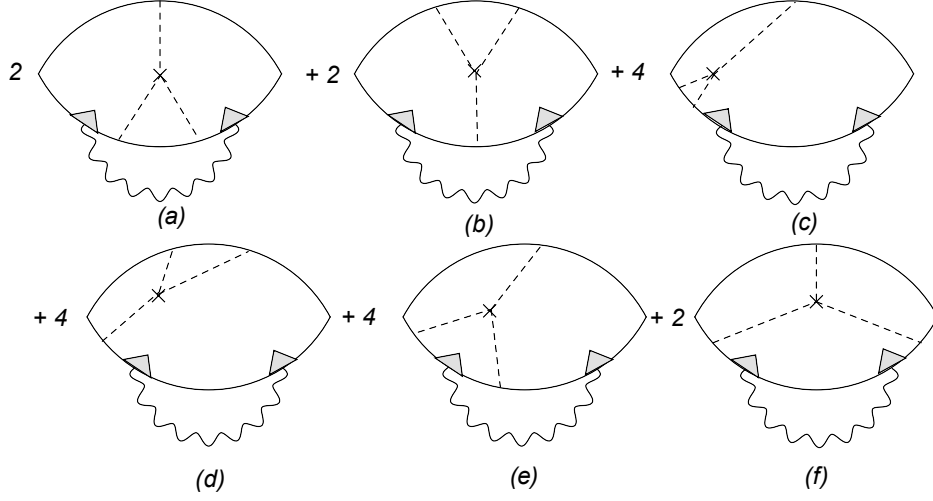
Figure 2: Diagrams for the density of states corrections to the anomalous Hall conductivity in the skew-scattering mechanism. The convention for the diagrammatic blocks is the same as in Fig. 1. The numerical coefficients in front of each diagram indicates the total number of possible rearrangements of skew impurity lines and fluctuation propagator line that lead to a similar contributions.
