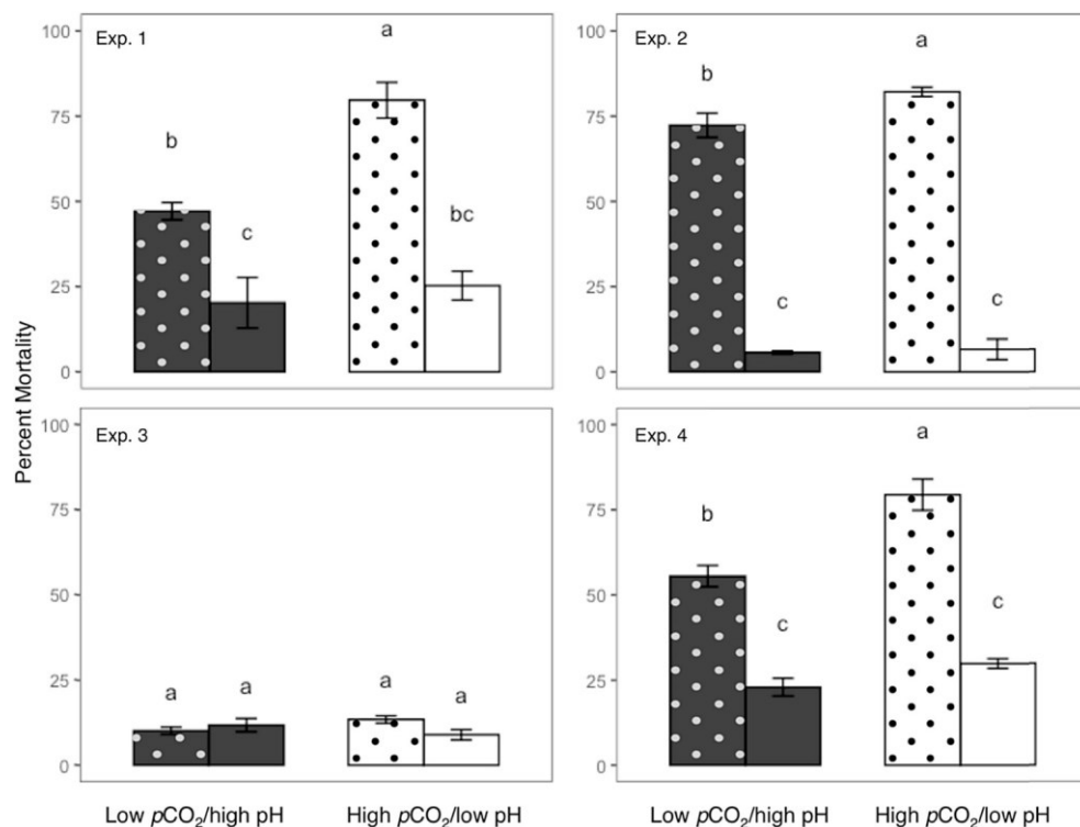
Fig. 3. Mortality of control (undotted) and bacteria-challenged (dotted) larval and juvenile clams (mean \pm standard error of the mean, n = 4 replicates). Different letters denote significantly different mortality levels between treatments within each experiment (two-way ANOVA, Tukey Kramer post hoc test, p < 0.05 ). Experiment 1: 24 h post challenge, 2-day old larvae, no \text{CO}_2 bubbling. Experiment 2: 24 h post challenge, 6-day old larvae exposed to bacteria with bubbling. Experiment 3: 96 h post challenge, 38 day old juvenile clams with bubbling. Experiment 4: 48 h post challenge, 33-day old juvenile clams without bubbling.
