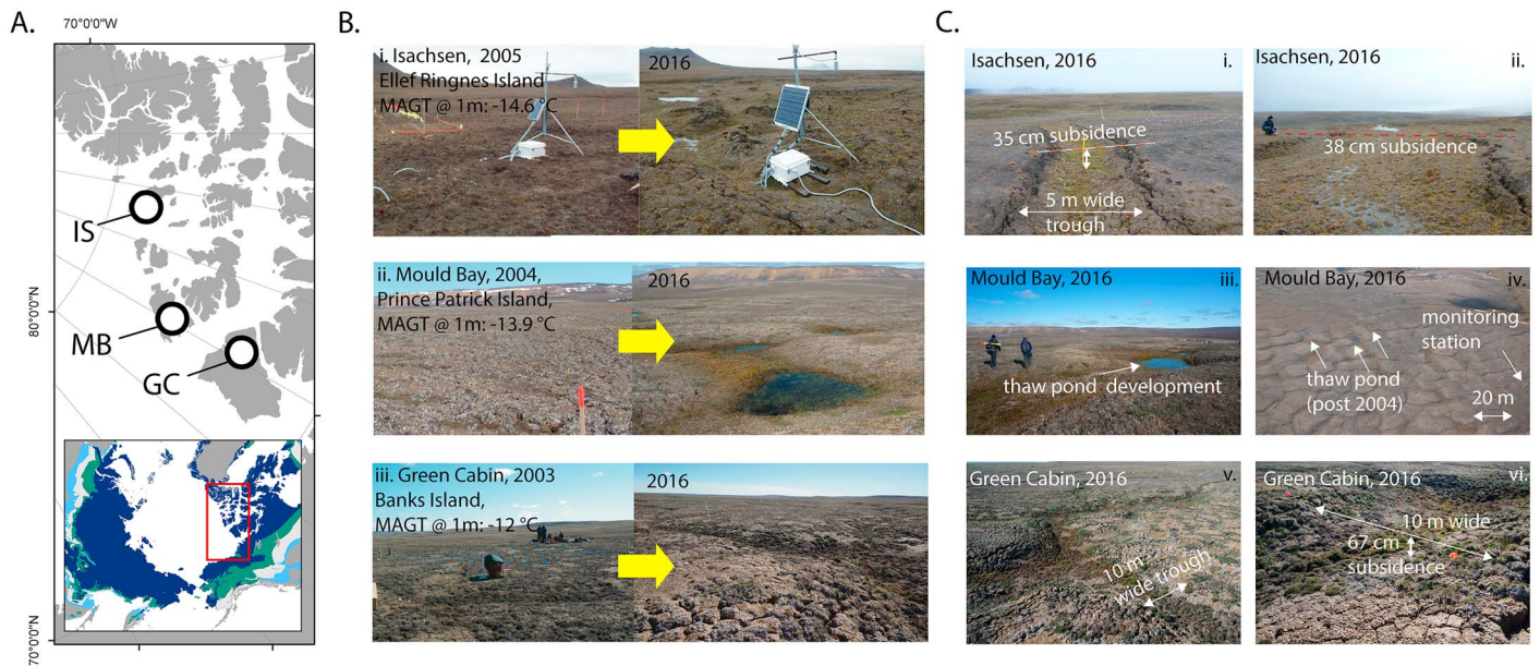
Figure 1. (a) Map of the study area showing permafrost monitoring site locations. (b) Examples of the even terrain at each site at the start of monitoring (2003, 2004, 2005) and the terrain after a decade of monitoring (2016). Thermokarst development was observed at all sites. (c) Examples of thermokarst topography and landforms observed at each site in 2016: (i and ii) subsidence and trough formation at Isachsen, (iii) trough formation and pond development at Mould Bay, and (iv) subsidence and trough formation at Green Cabin. All images are taken from within 500 m of the permafrost monitoring station with the exception of iv which was taken aerially but includes the monitoring station within the frame.
