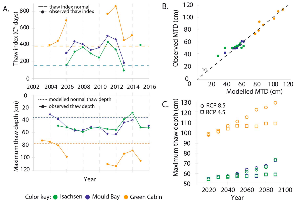
Figure 2. (a, top graph) TI (°C-days) through time for the three study sites. The dotted lines represent the thawing index normals (1979 to 2000; http://climate.weather.gc.ca/historical_data ; Everett, 1968) for each site. Time on the x axes is in calendar years. (bottom graph) Maximum thaw depth (cm) for each year at the three study sites. The dotted lines represent modeled historic maximum thaw depths calculated using the Stefan equation (equation (1)) and values derived from the TI normals shown in the top graph. (b) Comparison of observed maximum thaw depths and thaw depths modeled using the Stefan equation and A values (equation (2)) derived from observed maximum thaw depths. (c) Projected thaw depths for our three study sites under RCP 4.5 and 8.5. For all diagrams the symbology is as follows: Isachsen, green; Mould Bay, blue; Green Cabin, orange.
