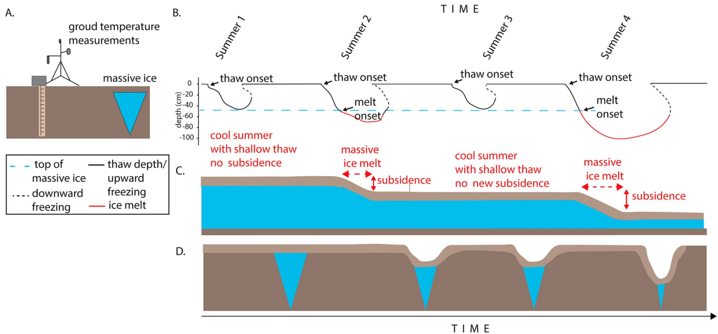
Figure 4. A schematic diagram of how summer thaw leads to rapid ice-wedge degradation. (a) An illustration of our monitoring station setup and source of ground temperature data in relation to near-surface massive ice. (b) A conceptual diagram illustrating thaw front dynamics based on measurements taken at our study sites. (c) A cross section of massive ice melt through time showing how protective sediment thickness remains the same despite active layer deepening, leading to cumulative melt throughout the thaw season. (d) A cross section of ice wedge thaw through three summers where the depth of thaw exceeded the sediment overburden above ice-wedge ice, and one cool summer where no additional subsidence occurs.
