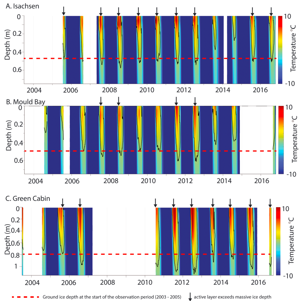
Figure 3. Thaw depth and temperature diagrams for (a) Isachsen, (b) Mould Bay, and (c) Green Cabin. Red dotted line shows ground ice depth at the start of the observation period. Black arrows indicate years where maximum thaw depth exceeds ground ice depth. The black continuous line is the 0 °C isotherm in the ground.
