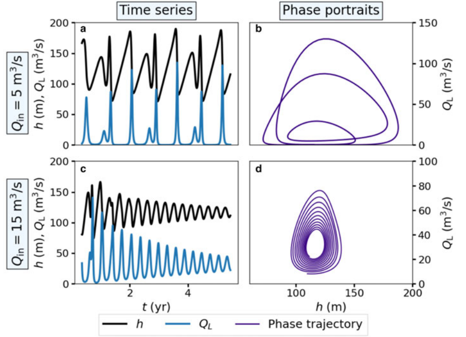
Fig. 6. Numerical simulations of a double-lake system for Q_{in} = 5 (a and b) and 15 \text{ m}^3 \text{ s}^{-1} (c and d). The relative downstream lake size is A_2^* = 1 and the scaled upstream channel length is L_1^* = 0.5 . The solutions for the downstream lake are plotted over time (a and c) and in Q_L - h phase space (b and d). The solutions for the upstream lake are not plotted because they are nearly identical to those in Fig. 2. Note that when Q_{in} = 15 \text{ m}^3 \text{ s}^{-1} (panels c and d), the discharge approaches the equilibrium value Q_L = 2Q_{in} . The dimensionless parameters are (a_m, a_c) = (66, 2900) (a and b) and (a_m, a_c) = (28, 967) (c and d).
