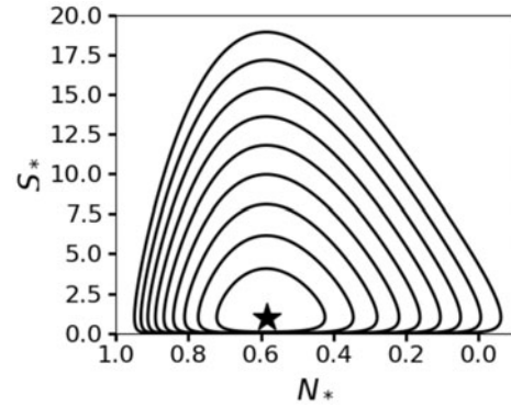
Fig. 11. Level curves of the Hamiltonian \mathcal{H}_1(\Phi, N_*) in Eqn (B11) plotted in the (S_*, N_*) -plane. We choose (a_m, a_c) = (30, 150) . The fixed point is noted by the black star.
