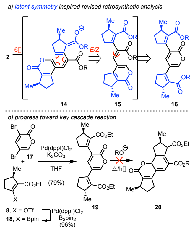
Scheme 3. Revised retrosynthetic analysis and preliminary attempts to initiate the cascade sequence.
