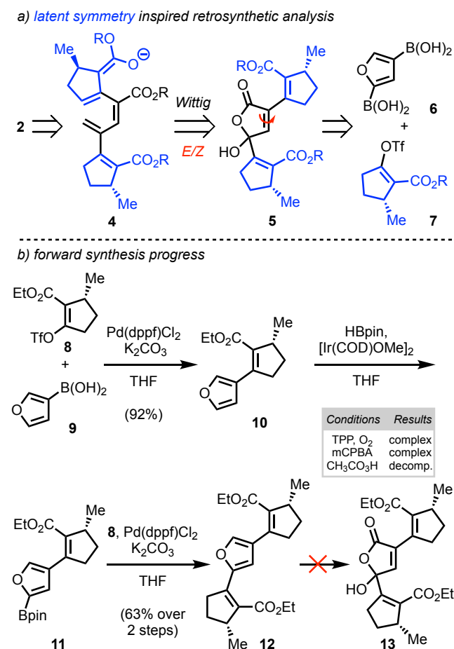
Scheme 2. Symmetry-inspired first generation approach.
