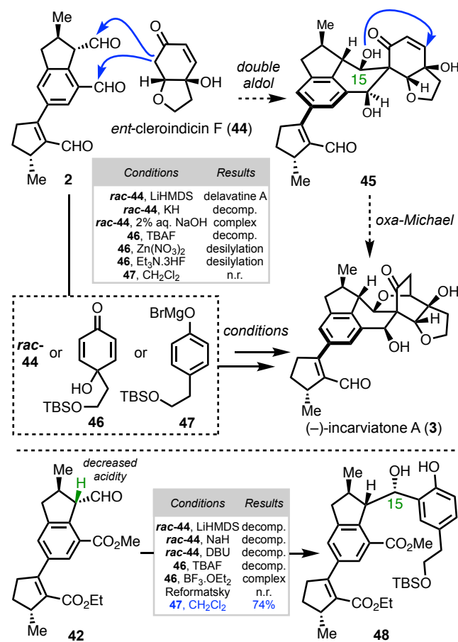
Scheme 11. Bioinspired attempts to synthesize incarviation A ( 3 ).
