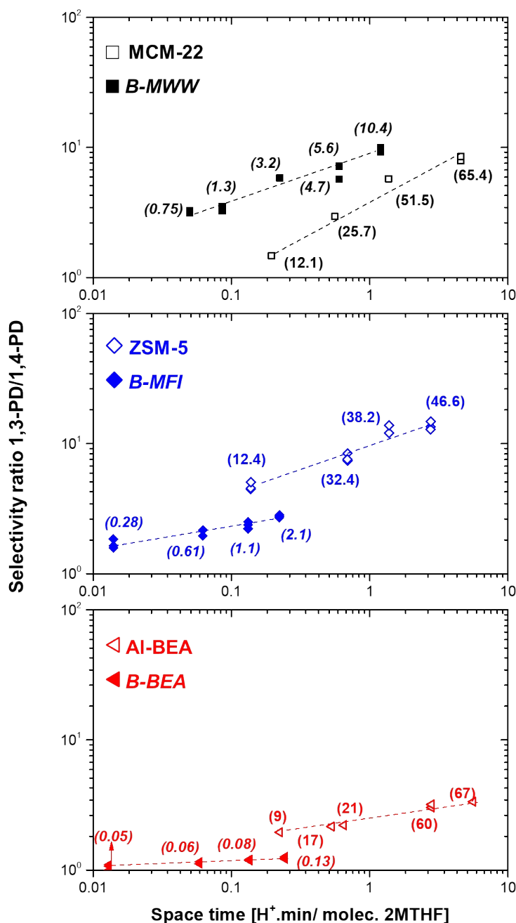
Figure 3. Measured selectivity ratios of 1,3-Pentadiene/1,4-Pentadiene as a function of reactor space-times over B-MWW (■, black), MCM-22 (□, black), B-MFI (◆, blue), ZSM-5 (◇, blue), B-BEA (◄, red), and Al-BEA (◁, red) (Reaction conditions: T=503 K, p_{2\text{-MTHF}} = 1.5-120 torr, Carrier gas (He) flowrate =60 sccm). The bracketed values are the corresponding conversion levels. Dashed lines are provided to guide the eye.
