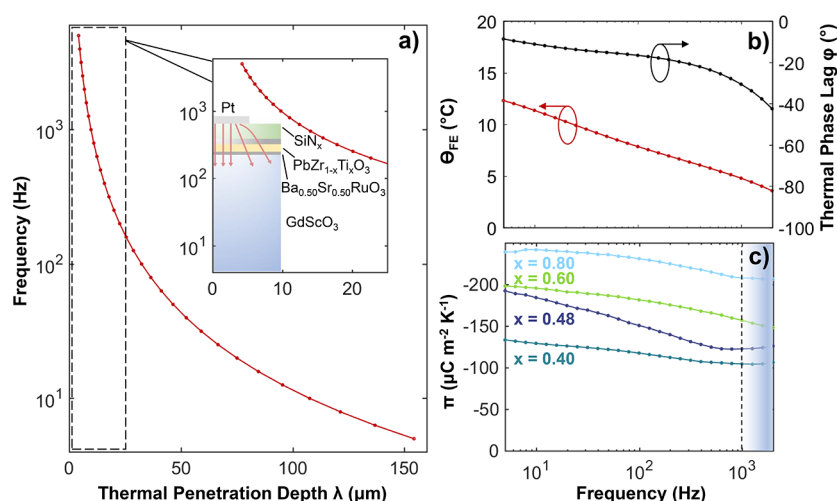
Figure 2. Thermal and secondary measurements of PbZr 1-x Ti x O 3 thin-films. (a) Calculated thermal penetration depth into the GdScO 3 substrate used to define the cutoff frequency for secondary contributions. Inset displays a schematic of the heat flux through the thin-film stack where the heater half width is approached at 1 kHz. (b) Temperature oscillation amplitude (left axis) and associated thermal phase lag (right axis) within the ferroelectric film as a function of heating frequency 1\omega . (c) Frequency dependence of the \pi displaying a suppressed secondary effect past \sim 1 kHz.
