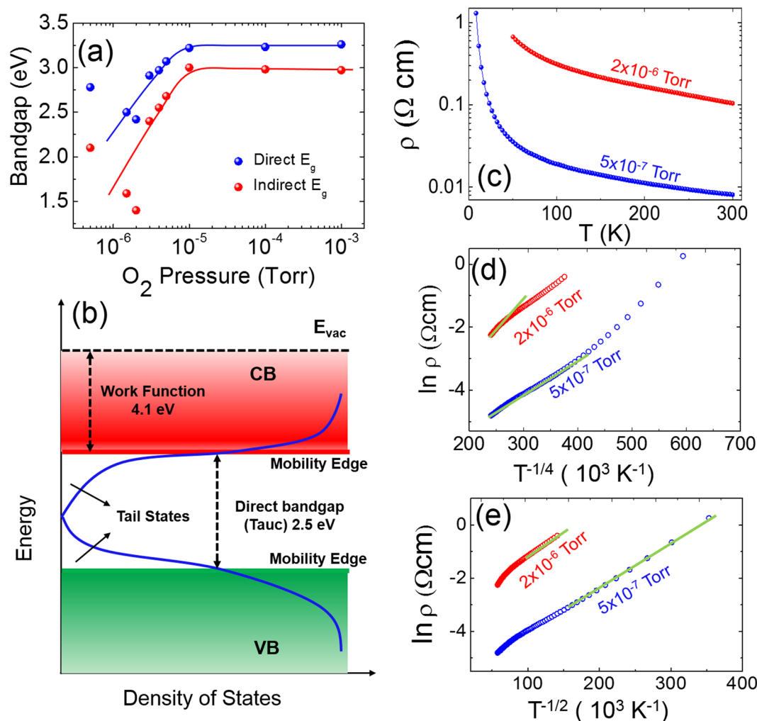
Figure 2. Band-gap and electrical conductivity of amorphous FDTO. (a) Direct and indirect bandgap obtained from Tauc plot for thin films of a-FDTO deposited at oxygen pressures ranging from 5 \times 10^{-7} Torr to 1 \times 10^{-3} Torr. (b) Schematic of band structure of a-FDTO film deposited at 2 \times 10^{-6} Torr showing the bandgap, work function, and mobility edges and tail states at the conduction and valence bands. (c) Resistivity as a function of temperature from 3 K to 300 K for two a-FDTO films deposited at two different oxygen pressures. Both curves show semiconductor behavior. (d), (e) Fit of temperature dependent resistivity to (d) 3-D variable range hopping model, showing good fit for both a-FDTO films above 100 K, and (e) 1-D variable range hopping model showing good fit for both films below 100 K.
