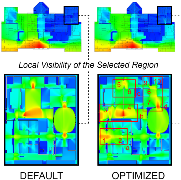
Fig. 7: Metropolitan Museum Design. We illustrate a visibility analysis of the whole museum and the optimization of a specific are of the layout with reduced visibility. We highlight the major improvements produced by IDOME: (a) enlarging the passage between zone 1 and zone 2 to create a centralized exposition space, which is better connected to the adjacent zones; (b) enlarging the size of zone 3 and 4 and improving their connection; (c) transforming zone 5 from a narrow corridor to a larger exposition space better connected to the surrounding zones; (d) improving the visual connectivity between zone 7, 8, 9 and 10.
