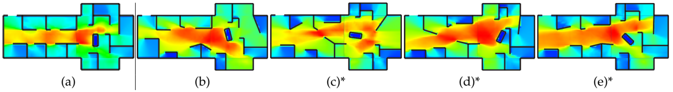
Fig. 6: Art gallery design. The diverse set of art gallery designs with combined spatial metric values displayed as heatmaps over the entirety of each design. Figure (a) is the original art gallery design. Figures (b-e) show the diversity members provided by the IDOME system for a particular environment parametrization. The (*)s identify the designs that six expert architects independently designated as preferred.
