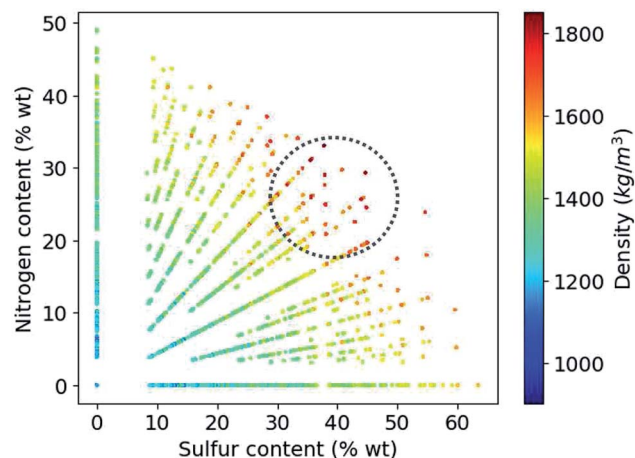
Fig. 6 Variation of density values as a function of weight percentage of sulfur and nitrogen in the molecules.
