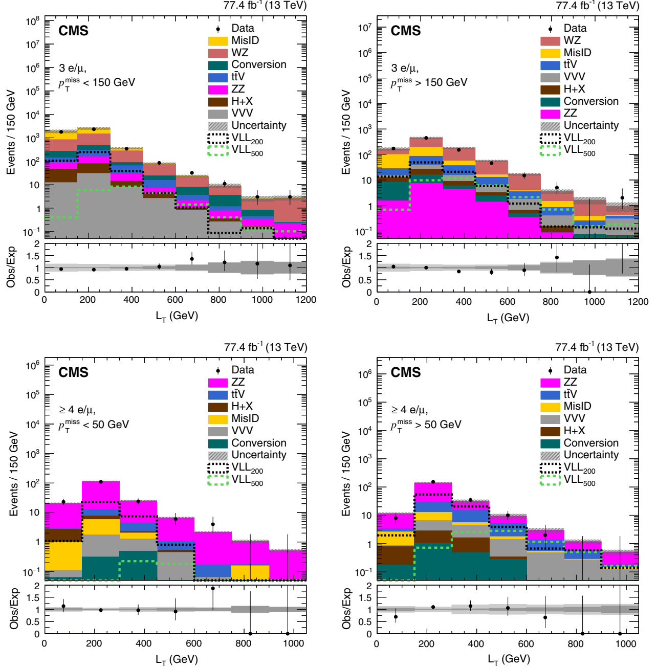
FIG. 4. The L_T distributions for the 3L signal regions with p_T^{\text{miss}} < 150 GeV (upper left) and p_T^{\text{miss}} > 150 GeV (upper right) and for the 4L signal regions with p_T^{\text{miss}} < 50 GeV (lower left) and p_T^{\text{miss}} > 50 GeV (lower right). The total SM background is shown as a stack of all contributing processes. The predictions for VLL signal models (the sum of all production and decay modes) with m_{\ell'/\ell''} = 200 and 500 GeV are shown as dashed lines. The hatched gray bands in the upper panels represent the total uncertainty in the expected background. The lower panels show the ratios of observed data to the total expected background. In the lower panels, the light gray band represents the combined statistical and systematic uncertainty in the expected background, while the dark gray band represents the statistical uncertainty only. The rightmost bins include the overflow events.
