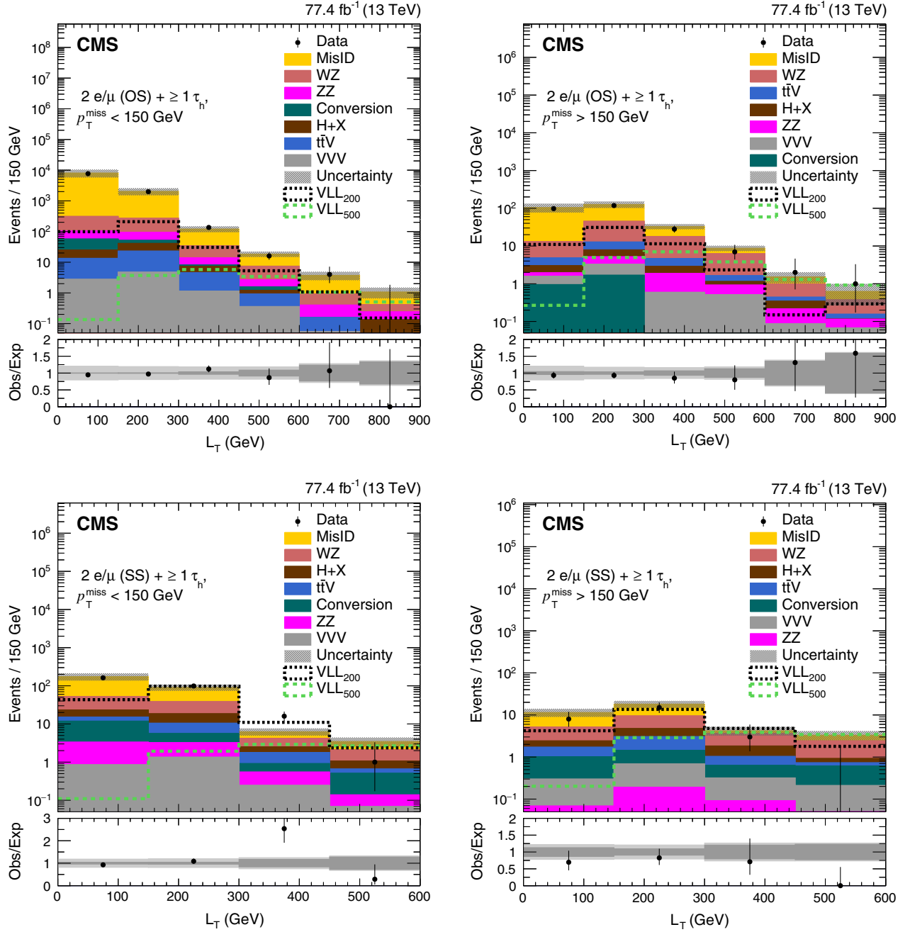
FIG. 5. The L_T distributions for the 2L1T OS signal regions with p_T^{\text{miss}} < 150 GeV (upper left) and p_T^{\text{miss}} > 150 GeV (upper right) and for the 2L1T SS signal regions with p_T^{\text{miss}} < 150 GeV (lower left) and p_T^{\text{miss}} > 150 GeV (lower right). The total SM background is shown as a stack of all contributing processes. The predictions for VLL signal models (sum of all production and decay modes) with m_{\tau'/\nu} = 200 and 500 GeV are also shown as dashed lines. The hatched gray bands in the upper panels represent the total uncertainty in the expected background. The lower panels show the ratios of observed data to the total expected background. In the lower panels, the light gray band represents the combined statistical and systematic uncertainty in the expected background, while the dark gray band represents the statistical uncertainty only. The rightmost bins include the overflow events.
