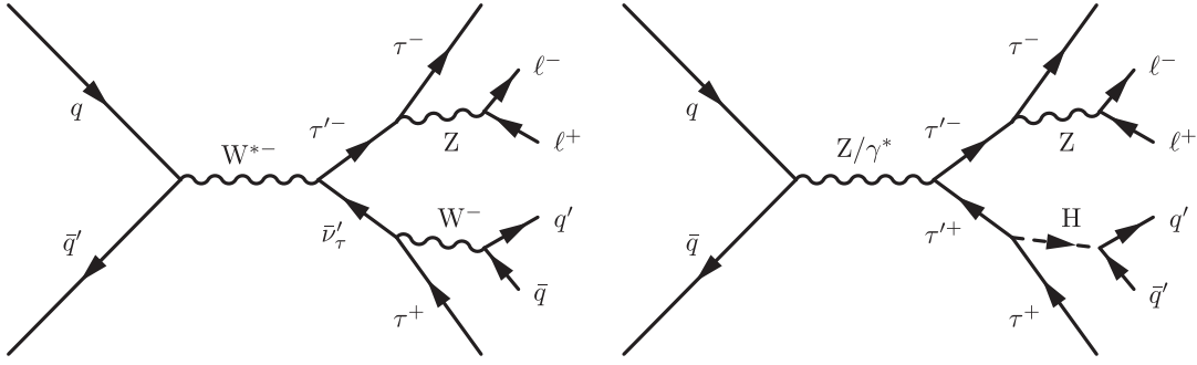
FIG. 1. Two illustrative leading-order Feynman diagrams for associated production of \tau' with a \nu'_{\tau} (left) and for pair production of \tau' (right) and possible subsequent decay chains that result in a multilepton final state.
