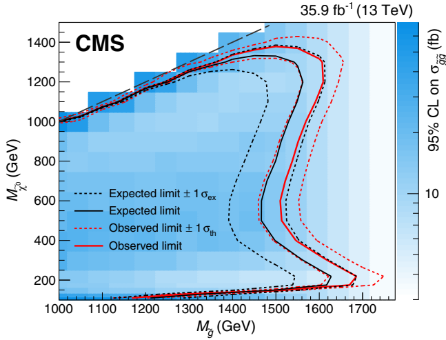
FIG. 4. The upper limit at 95% confidence level on the \tilde{g} pair production cross section as a function of \tilde{g} and \tilde{\chi}_1^0 masses. The region enclosed by the red (lighter) solid line is excluded. The black (darker) solid line presents the expected excluded area. The uncertainty in the observed limit corresponds to the theoretical uncertainties in the signal cross section. Exclusion in the low \tilde{\chi}_1^0 and high \tilde{g} mass region is a result of the implementation of the substructure techniques.
