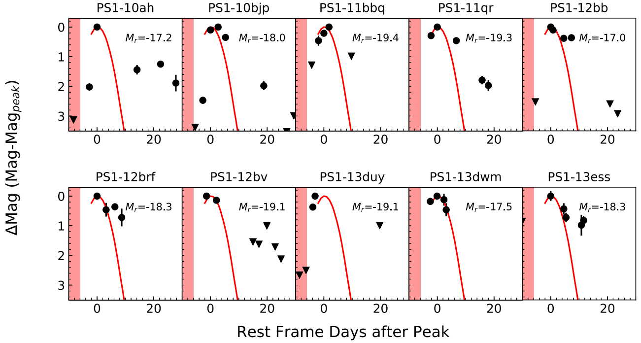
Figure 9. SDSS r -band LC of SN 2019bkc (red line) compared to those of rapidly evolving transients from Pan-STARRS1 reported in Drout et al. (2014). The estimated most likely explosion date of SN 2019bkc is within the vertical shaded region in red.
