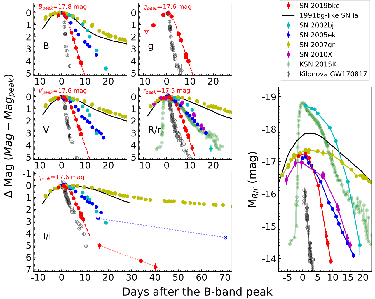
Figure 2. B -, V -, g -, R/r -, and I/i -band LCs of SN 2019bkc compared with the fast-evolving Type I SNe 2002bj, 2005ek, and 2010X, the fastest-declining 1991bg-like Type Ia, the Type Ic SN 2007gr, and the fast transient KSN 2015K (in Kepmag) found by Kepler and the kilonova GW 170817. The left panels normalize the LCs to the peak brightness, while the right panel shows the absolute R/r -band magnitudes. The dashed lines represent the third-order polynomial fit to the LCs used to estimate the peak (displayed up to +4 days) and the linear fits between +4 and +10 days used to estimate the decline-rate parameters in Section 3.1. The red and blue dotted line is the best-fit straight line for the late-time i -band LC of 2019bkc and 2005ek, respectively.
