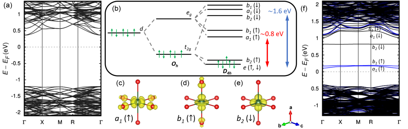
FIG. 4. (a) Pristine band structure of Co 3 O 4 with a 224 atom supercell (primitive cell band structure shown in SM, Fig. S5). (b) Hole polarons create a low-spin (LS) d^5 configuration at Co(O) along with a Jahn-Teller (JT) distortion which results in a D_{4h} configuration and the creation of several midgap states. (c)–(e) Wave function isosurface plots (yellow cloud) of the three polaron induced states under hole formation of a_1(\uparrow)(d_{x^2-y^2}) , b_1(\uparrow)(d_{z^2}) , and b_2(\downarrow)(d_{xy}) character, respectively. Isosurface plots use a cutoff value of 10% the maximum. (f) Band structure of Co 3 O 4 with a hole polaron which shows several induced gap states (blue = spin up; black = spin down).
