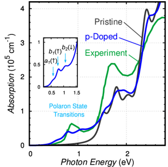
FIG. 5. Optical absorption of Co 3 O 4 in the pristine system (black) and the p -doped system (blue). Notably, only p -type doping, i.e., the formation of holes, will cause midgap transitions below 1.6 eV, in agreement with experimental optical spectrum of Co 3 O 4 shown in green [49]. The inset image displays the midgap transitions which are labeled according to the states formed from hole polaron formation as in Fig. 4. (Theoretical spectrum is an average of spectra with light polarized in the [100], [010], and [001] directions.)
