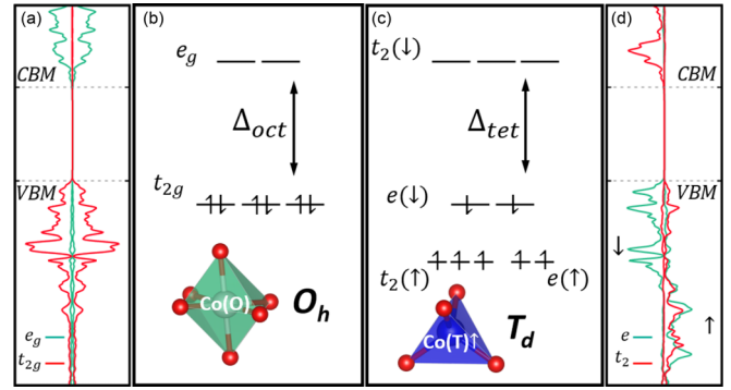
FIG. 3. (a) Projected density of states (PDOS) of Co(O) on t_{2g} and e_g orbitals. Schematic representation of the electronic configuration of (b) octahedral \text{Co}^{3+} and (c) tetrahedral \text{Co}^{2+} in \text{Co}_3\text{O}_4 due to a crystal field splitting ( \Delta_{\text{oct}} and \Delta_{\text{tet}} , respectively). (d) PDOS of Co(T) on t_2 and e orbitals. All the PDOS were computed with DFT+ U .
