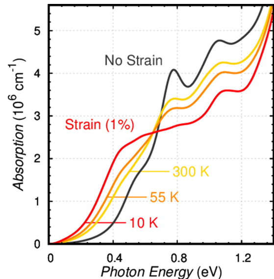
FIG. 6. Optical absorption of p -doped \text{Co}_3\text{O}_4 under 1% uniaxial tensile strain along the [100] direction. Temperature dependence determines the probability for which direction the Jahn-Teller elongation will occur (as the degeneracy is removed under strain) and results in a redshift of optical peaks related to the hole polaron.
