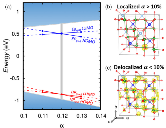
FIG. 2. (a) Generalized Koopmans' condition for electron polaron (EP) and hole polaron (HP) in \text{Co}_3\text{O}_4 . The exact exchange \alpha for the PBE0( \alpha ) method is varied until the condition \text{HOMO}_q = \text{LUMO}_{q+1} (at fixed geometry where polaron has formed) is met. In both cases, we find that at an exact exchange of 0.12 Koopmans' condition is satisfied. The corresponding pristine gap is computed to be 1.70 eV. (b) Localized and (c) delocalized hole wave function, subject to the value of the exact exchange. Isosurface plots use a cutoff of 10% the maximum.
