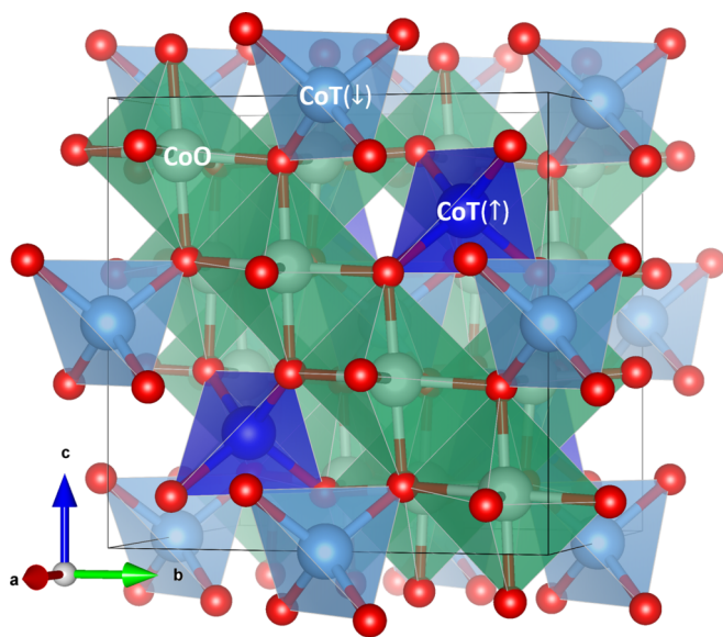
FIG. 1. Normal spinel atomic structure of \text{Co}_3\text{O}_4 . Octahedral Co are shown in green, tetrahedral Co are shown in blue/light blue (distinguishing spin polarization direction), and O are shown in red.
