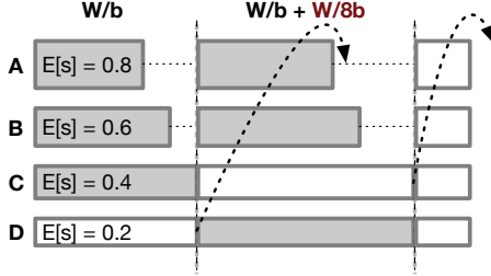
Fig. 11. Parallel job using FSP on transient servers.
