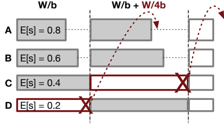
Fig. 9. Parallel job using partial barriers on transient servers.
