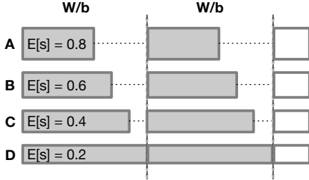
Fig. 3. Parallel job using BSP on transient servers.
