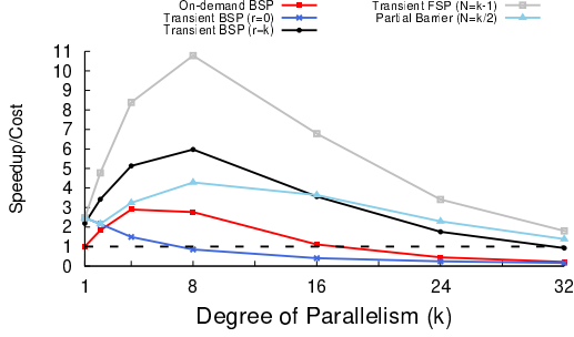
Fig. 13. The speedup/cost ratio for executing our baseline parallel job for different straggler mitigation techniques on on-demand and transient servers.
