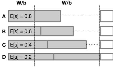
Fig. 7. Parallel job using bounded staleness on transient servers.
