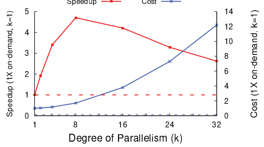
Fig. 2. Speedup and cost of executing our representative parallel job using BSP on on-demand cloud servers as the degree of parallelism increases.
