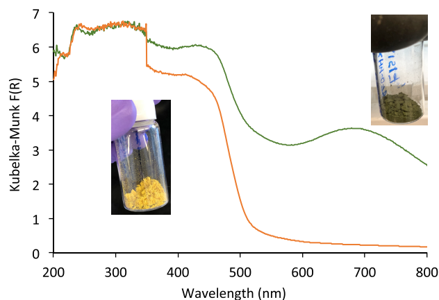
Figure 3. Kubelka–Munk diffuse reflectance spectra and photographs of DBA-COF 5 (orange) and Ni-DBA-2D-COF (green).
