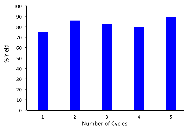
Figure 4. Recyclability of Ni-DBA-2D-COF after reductively cleaving 2-(methylthio)naphthalene (1c) at 130 °C using dimethylethylsilane as the reducing agent.
