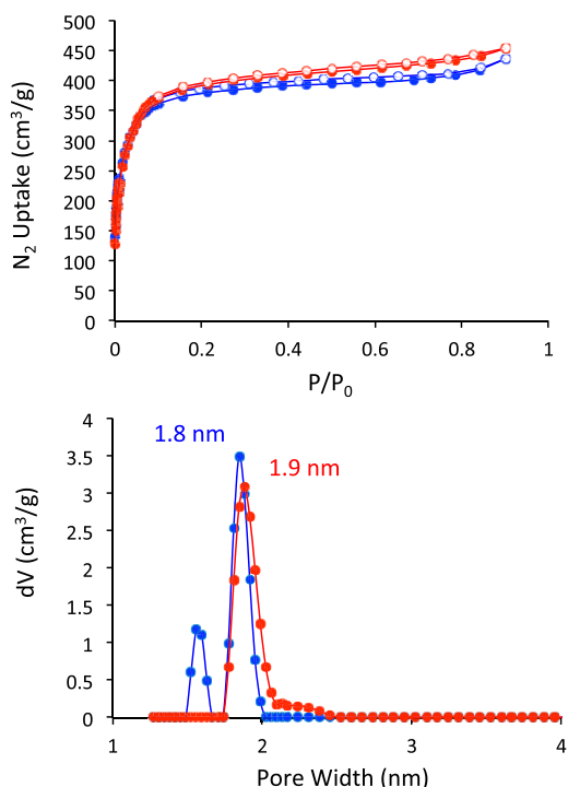
Figure 1. Nitrogen adsorption/desorption isotherms (top) and NLDFT pore size distributions (bottom) for DBA-COF 5 (red) and Ni-DBA-2D-COF (blue) measured at 77 K.
