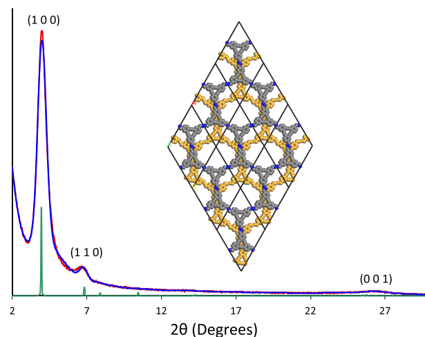
Figure 2. Indexed experimental (red) and Pawley refined (blue) PXRD patterns of DBA-COF 5 compared to the simulated hexagonal unit cell (green) with an offset of 9 Å and views along the x and y directions.
