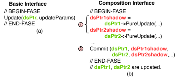
Figure 6. Failure-atomic Code Sections (FASEs) with MOD datastructures using (a) Basic interface to update one datastructure and (b) Composition interface to atomically update multiple datastructures with (1) Update and (2) Commit.
