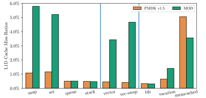
Figure 11. L1D Cache miss ratios for PM workloads.
