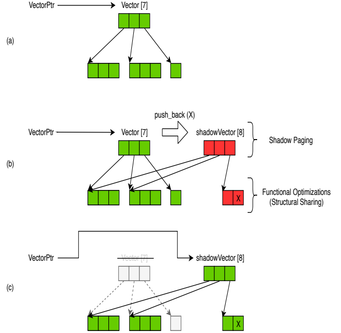
Figure 5. Functional Shadowing in action on (a) MOD vector. (b) push_back operation creates a shadow that reuses data from the original. (c) Application proceeds with shadow and old data is reclaimed.
