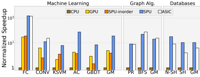
Figure 15: Overall Performance
