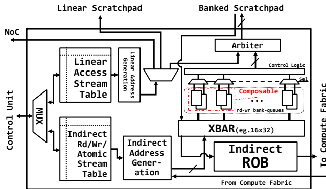
Figure 9: Scratchpad Controller
