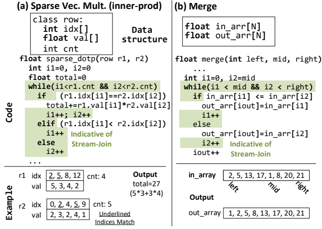
Figure 2: Example Stream-Join Algorithms
