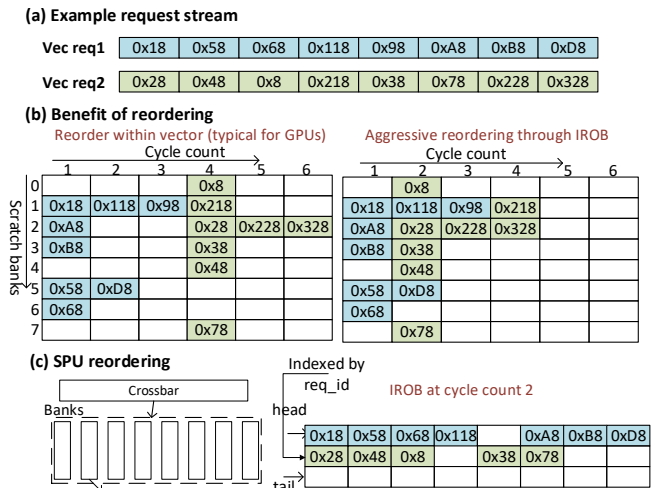
Figure 11: Functioning of IROB. (bits<6..4> indicate bank number)
