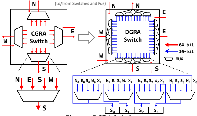
Figure 7: DGRA Switch
