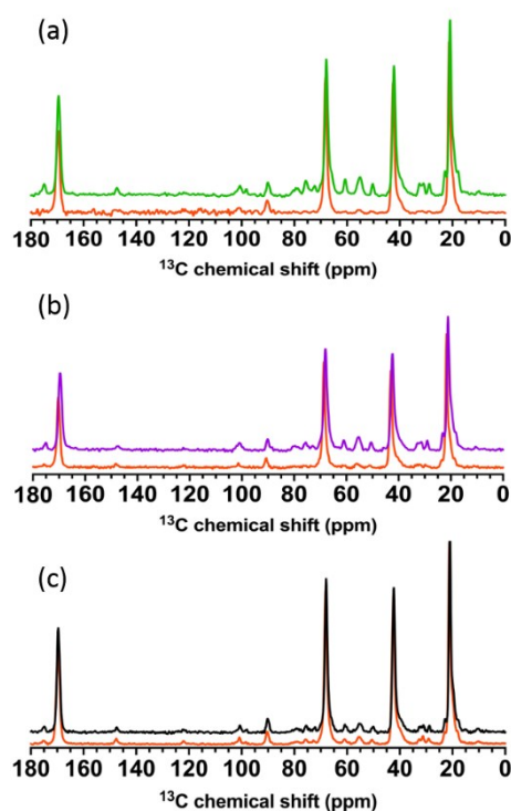
Fig. 9 Solid-state 13 C-NMR spectra of (a) wild type, (b) \Delta tagE , and (c) \Delta dltA where the orange trace shows the result of 34 nM bPEI-AuNPs.
