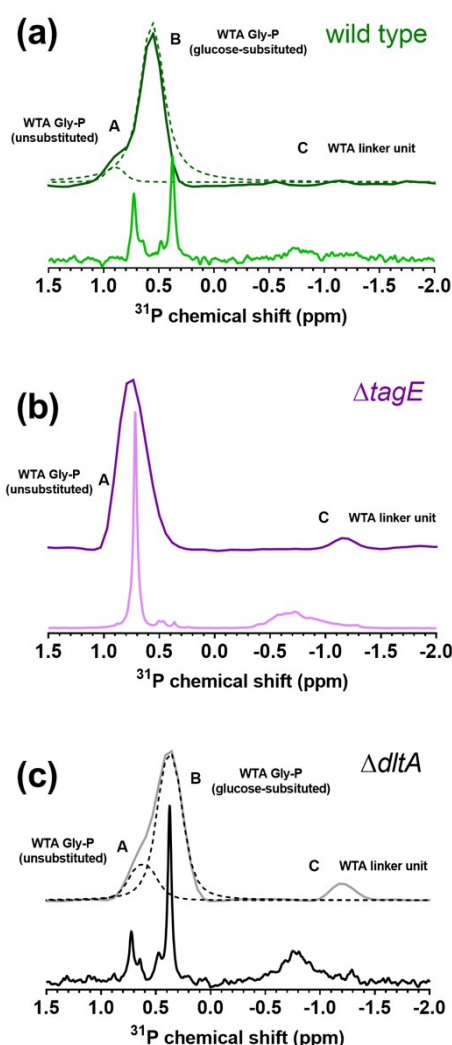
Fig. 4 Solution and solid-state ^{31}\text{P} -NMR spectra for (a) wild type, (b) \Delta tagE , and (c) \Delta dltA strains of Bacillus subtilis . Dashed lines in the solid-state spectra indicate deconvoluted peaks. Peak A reflects unsubstituted glycerolphosphate groups, peak B is due to glucose-substituted glycerolphosphate, and peak C is assigned to phosphorus in the linker unit. Sodium phosphate (at 2.5 ppm) and hexamethylphosphoramide (at 29.97 ppm) were used as internal standards for the solution and solid-state spectra, respectively.
