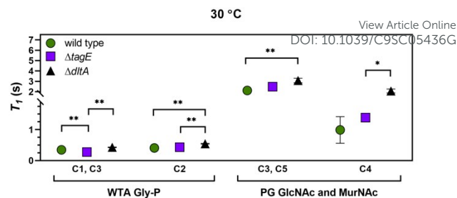
Fig. 6 T_1 relaxation time constants at 30 °C for the indicated ^{13}\text{C} resonances of sacculi from wild type, \Delta tagE , and \Delta dltA strains of B. subtilis : GlcNAc C3 and MurNAc C5 of peptidoglycan, GlcNAc and MurNAc C4 of peptidoglycan, glycerolphosphate C1 and C3 of wall teichoic acids, and glycerolphosphate C2 of wall teichoic acids. Non-linear fit statistical significance: *, p < 0.05 ; **, p < 0.01 . Error bars represent standard error in non-linear fitting from T_1 relaxation time equation. See Fig S6 for T_1 relaxation times for other temperatures. Abbreviations: GlcNAc, N -acetylglucosamine; MurNAc, N -acetylmuramic acid.
