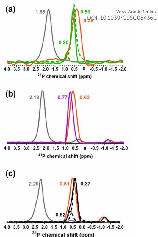
Fig. 8 Solid-state 31 P-NMR spectra for the (a) wild type (green), (b) \Delta tagE (purple), and (c) \Delta dltA (black) strains before and after exposure to 34 nM bPEI-AuNPs and 29.12 \mu M free bPEI polymer. In (a) and (c), deconvoluted spectra are shown with dashed lines. The orange traces reflect phosphorus signals upon interaction with 34 nM AuNPs. Grey traces correspond to sacculi exposed to 29.12 \mu M free bPEI polymer, the estimated amount of free polymer in a 34 nM AuNP solution. Numerical values in green, purple, or black (sacculi for each strain), orange (with AuNPs), and grey (with free bPEI polymer) are the corresponding peak shifts for predominant peaks and deconvoluted shoulders.
