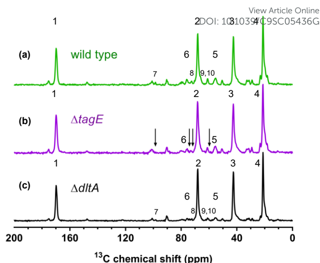
Fig. 5 Solid-state ^{13}\text{C} -NMR spectra of sacculi from (a) wild type, (b) \Delta tagE , and (c) \Delta dltA strains of Bacillus subtilis . Arrows indicate the absence of the glucose peak in the \Delta tagE strain. The peaks are assigned as follows: (1) carbonyl carbons in peptidoglycan amino acid and amino sugar residues and in WTA linker unit amino sugar residues; (2) C3 in the peptidoglycan amino sugar residues; (3) C2 in the peptidoglycan and WTA linker unit amino sugar residues; (4) methyl groups in the peptidoglycan and WTA linker unit amino sugar residues; (5) glycerol C1 and C3; (6) glycerol C2; (7) C1 from Glc; (8) C2, C3, and C5 from Glc; (9) C4 from Glc; and (10) C6 from Glc.
