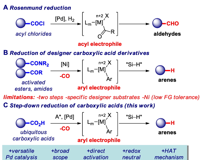
Fig. 1 (a) Transition-metal-catalyzed reduction of carboxylic acids.
