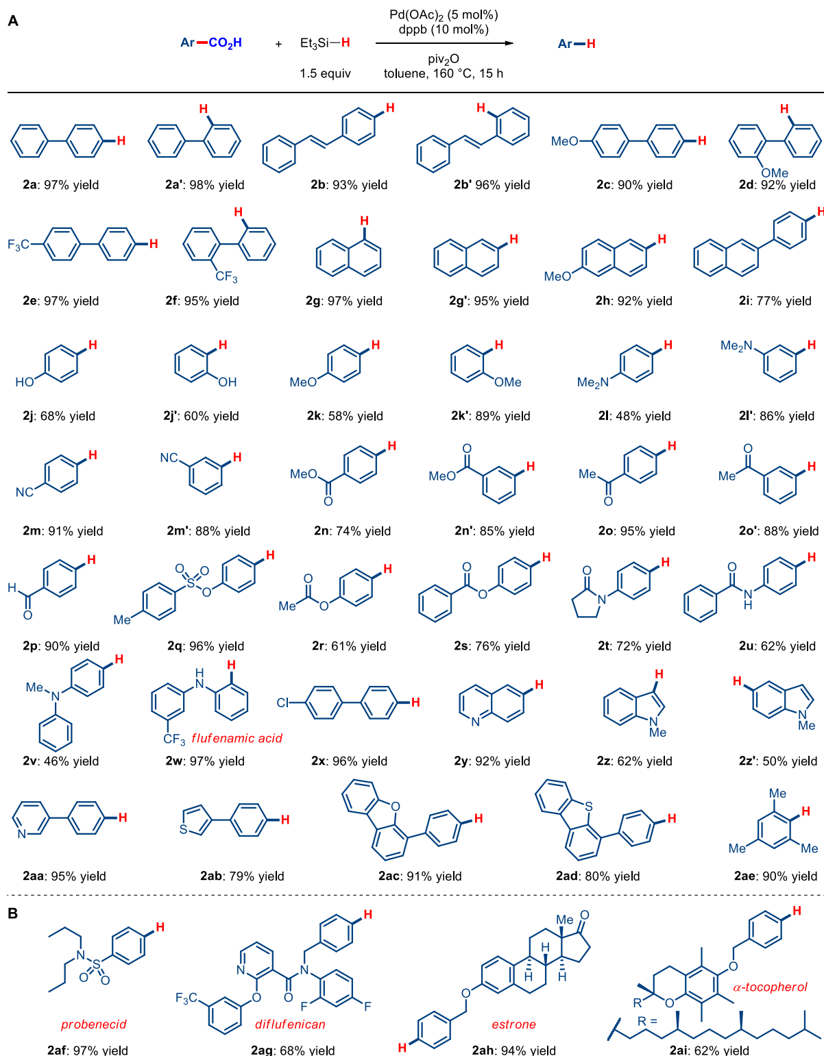
Fig. 2. Scope of decarbonylative reduction of carboxylic acids. Conditions: carboxylic acid (1.0 equiv), \text{Pd(OAc)}_2 (5 mol%), dppb (10 mol%), \text{Et}_3\text{SiH} (1.5 equiv), \text{piv}_2\text{O} (1.5 equiv), toluene, 160 °C, 15 h. Dppb = 1,4-bis(diphenylphosphino)butane; piv = pivaloyl. See SI for details.
