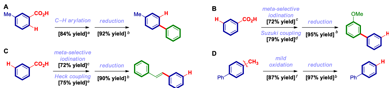
Fig. 3 Synthetic applications. a PhI, [Ru( p -cym)Cl 2 ] 2 , PCy 3 HBF 4 , K 2 CO 3 , NMP, 100 °C. b Standard conditions. c I 2 , NaIO 4 , H 2 SO 4 , 23 °C. d 3-MeO-C 6 H 4 -B(OH) 2 , Pd 2 (dba) 3 , SPhos, K 3 PO 4 , PhMe, 100 °C. e PhCH=CH 2 , Pd 2 (dba) 3 , Pt-Bu 3 HBF 4 , Et 3 N, dioxane, 23 °C. f KMnO 4 , Na 2 CO 3 , H 2 O, 120 °C.
