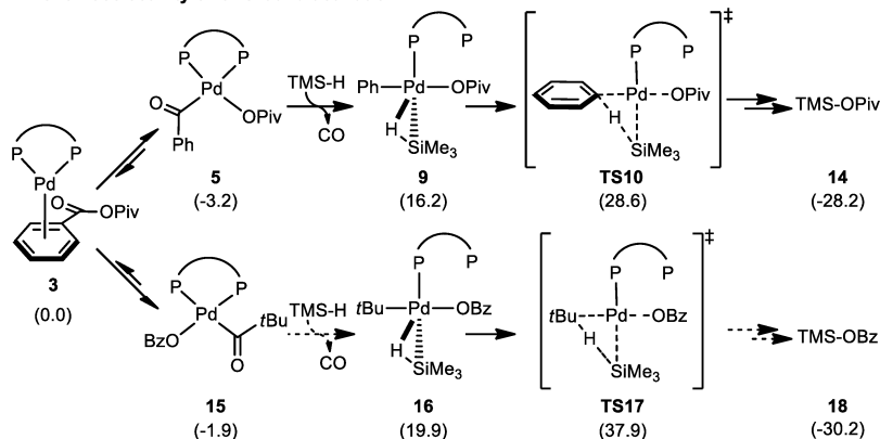
Fig. 4 DFT-calculated reaction energy profile and chemoselectivity of C–O bond activation of [Pd(dppb)]-catalyzed decarbonylative reduction of benzoic pivalic anhydride. See SI for computational details.
