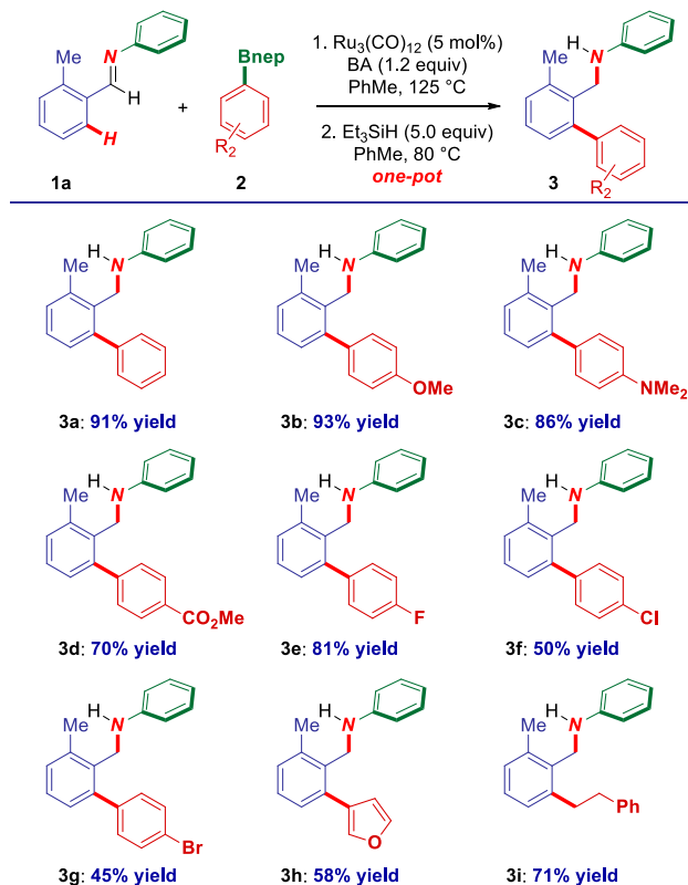
Scheme 1 Ruthenium(0) Sequential Catalysis: Direct C–H Arylation/Hydrosilylation a,b
