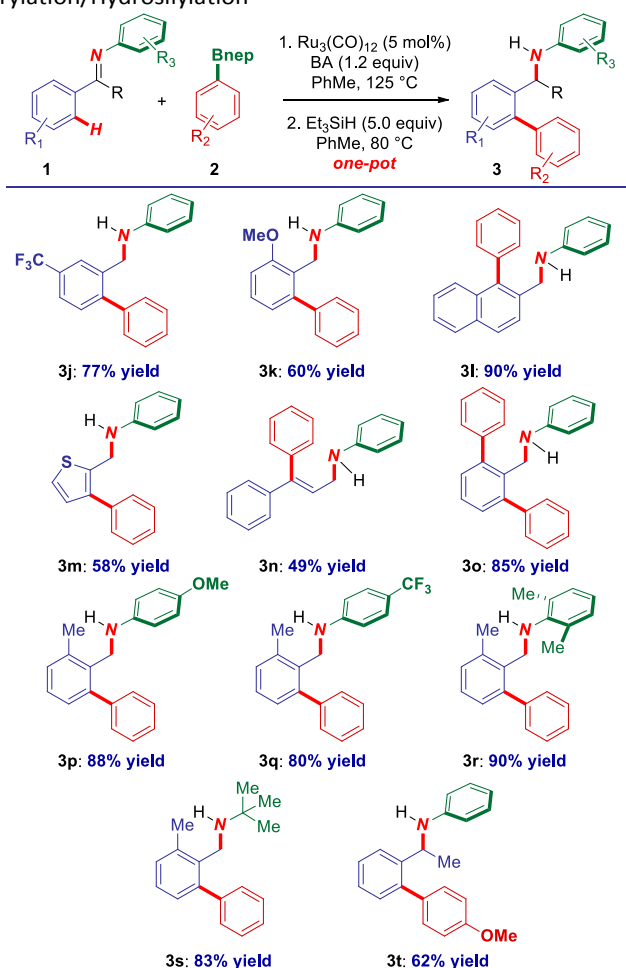
Scheme 2 Ruthenium(0) Sequential Catalysis: Direct C–H Arylation/Hydrosilylation a,b
