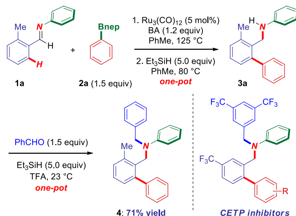
Scheme 4 Three-Component Ru(0)-Catalyzed Arylation/Reduction via In Situ Imine Synthesis
