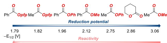
Figure 2. Redox potentials of O -ketyl precursors. a See SI for details. a Note that \text{MeCO}_2\text{pfp} derived from unactivated alkyl precursor is characterized by a lower redox potential ( E_{1/2} = -1.82 V) than \text{PhCO}_2\text{Me} derived from activated benzoic acid ( E_{1/2} = -2.12 V).
