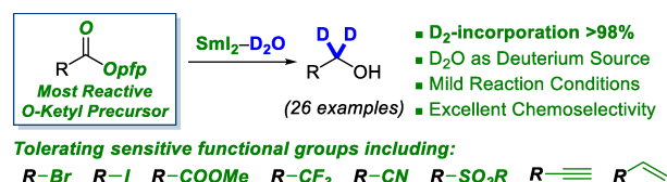
Figure 1. Reductive deuteration of esters: (a) traditional method; (b) previous studies; (b) this work: pentafluorophenyl (pfp) esters as the most reactive precursors to O -ketyl radicals.
