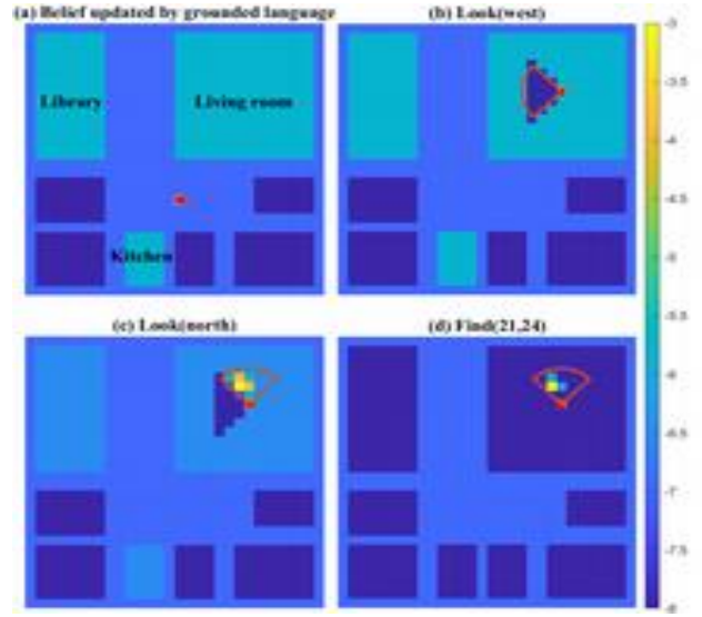
Fig. 1: The agent (red dot) must find the locations of one or more objects (yellow). (a) The belief after a language observation “Find the mugs in the library, living room, or kitchen.” (b) and (c) show the belief after a sensor observations via Look actions. (d) The agent’s belief converges to the true object location after a sequence of actions. (Probabilities in log scale.)
