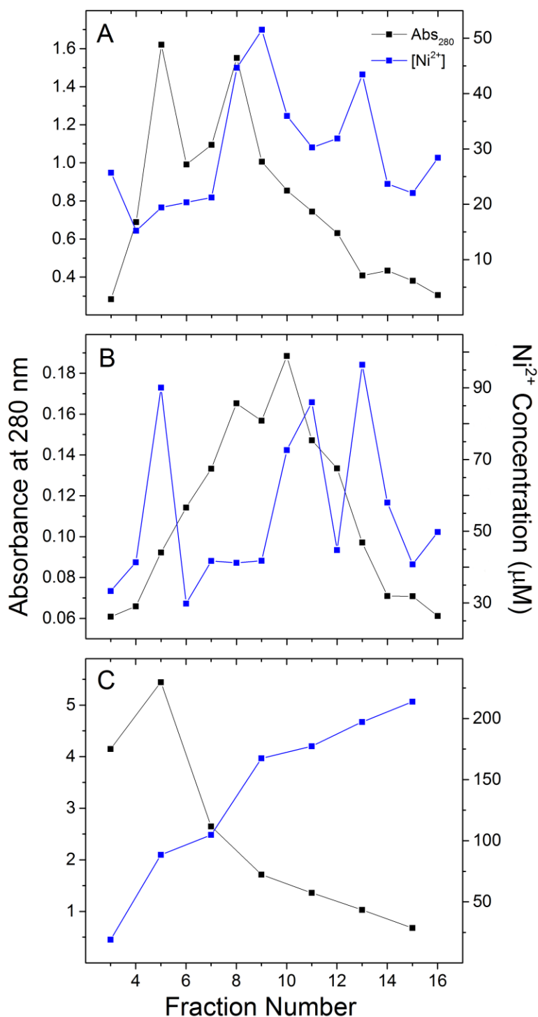
Figure 3. Ni 2+ quantification for 3 representative His-tag proteins. Protein and Ni 2+ elution profiles for (A) MSP1E3D1, (B) MSP2N2, and (C) GSU0105. Protein elution was performed using 300 mM, 300 mM, and 500 mM imidazole, respectively. Ni 2+ quantification was performed in 20 mM Tris, pH 7.5.
