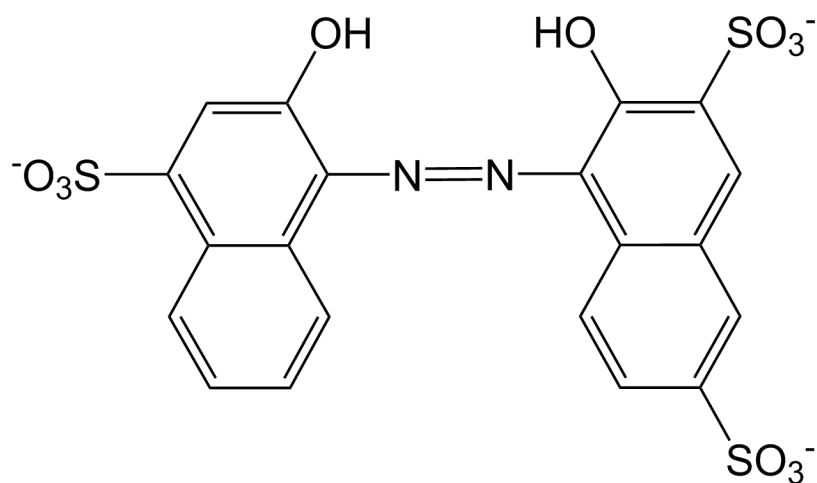
Figure 1. Structure of hydroxynaphthol blue (HNB). In the functional pH range of the assay, all sulfonate groups and one of the hydroxyl groups are ionized.
