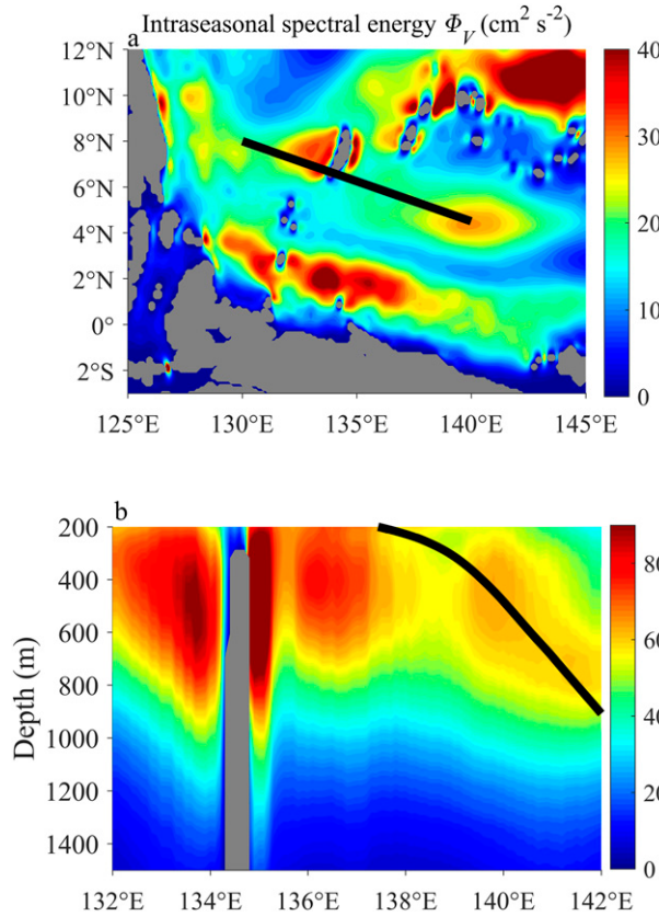
FIG. 9. (a) Horizontal distribution of the intraseasonal spectral energy for 50-day period at 1200-m depth based on OFES outputs. (b) The vertical section of the intraseasonal spectral energy along the black line in (a), representing the energy propagating path. In (b), the black solid line denotes the ray path of the first meridional mode short Rossby wave based on Eq. (7). The gray area indicates the geometry.
