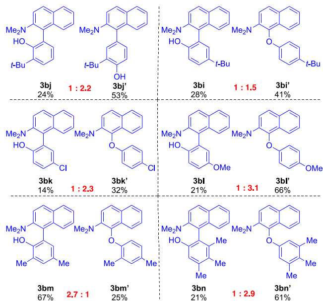
Figure 5. Couplings of N,N -dimethyl-2-aminonaphthalene with two outcomes (C–C ortho vs C–C para or C–C vs C–O; blue compounds are new compounds, not previously reported).
