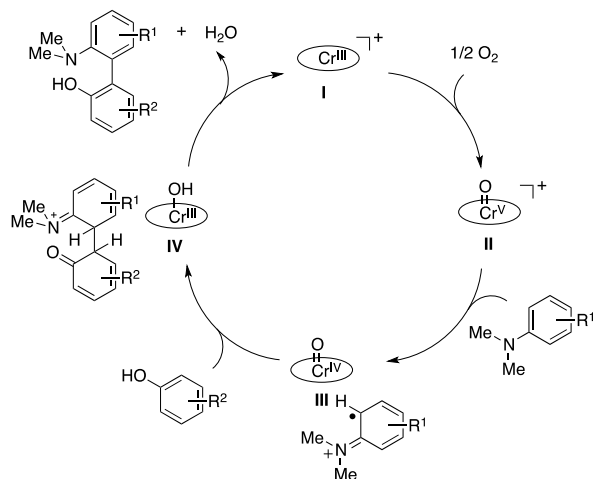
Figure 6. Proposed catalytic cycle for oxidative cross-coupling.
