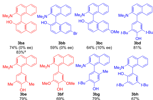
Figure 3. Couplings of N,N -dimethyl-2-aminonaphthalene using the conditions in eq 2. (Blue compounds are new compounds, not previously reported.) a Isolated yield on a 1.0 mmol scale.
