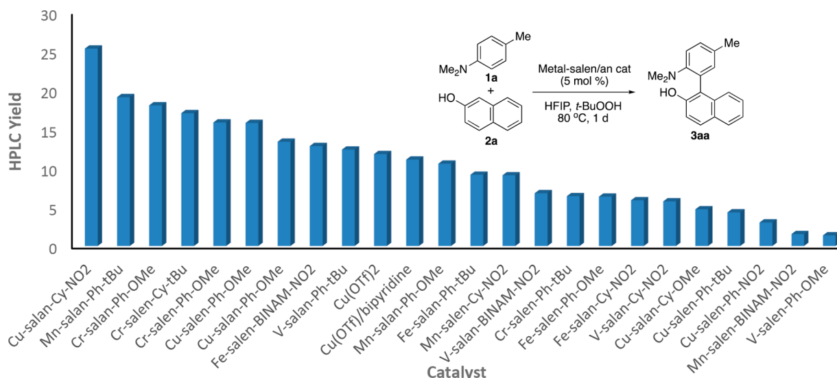
Figure 2. High-throughput experimentation results for the catalyst library screen (internal standard = 4,4'-di- tert -butylbiphenyl).
