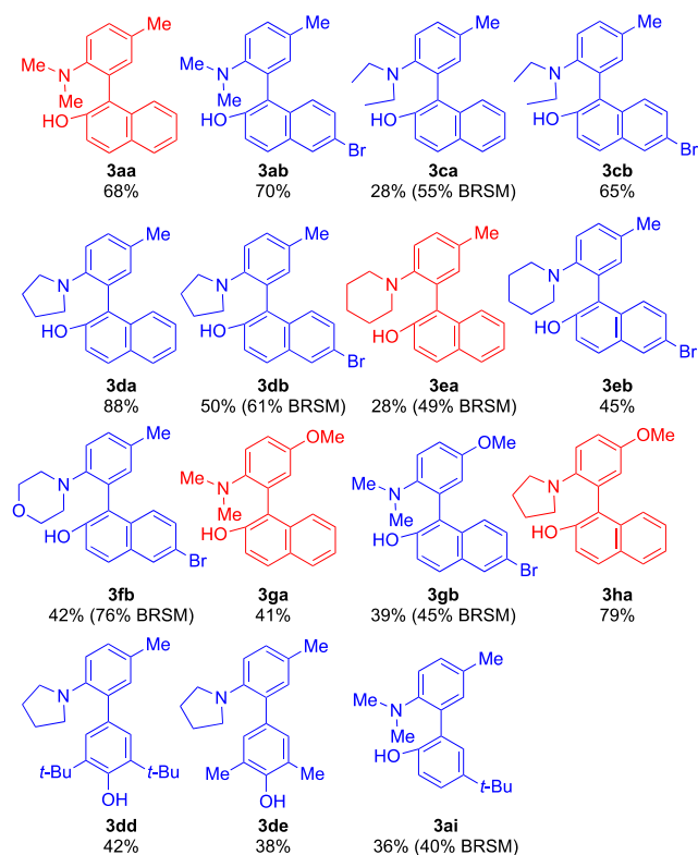
Figure 4. Couplings of anilines using the conditions in eq 2 (BRSM = based on recovered starting material; blue compounds are new compounds, not previously reported).
