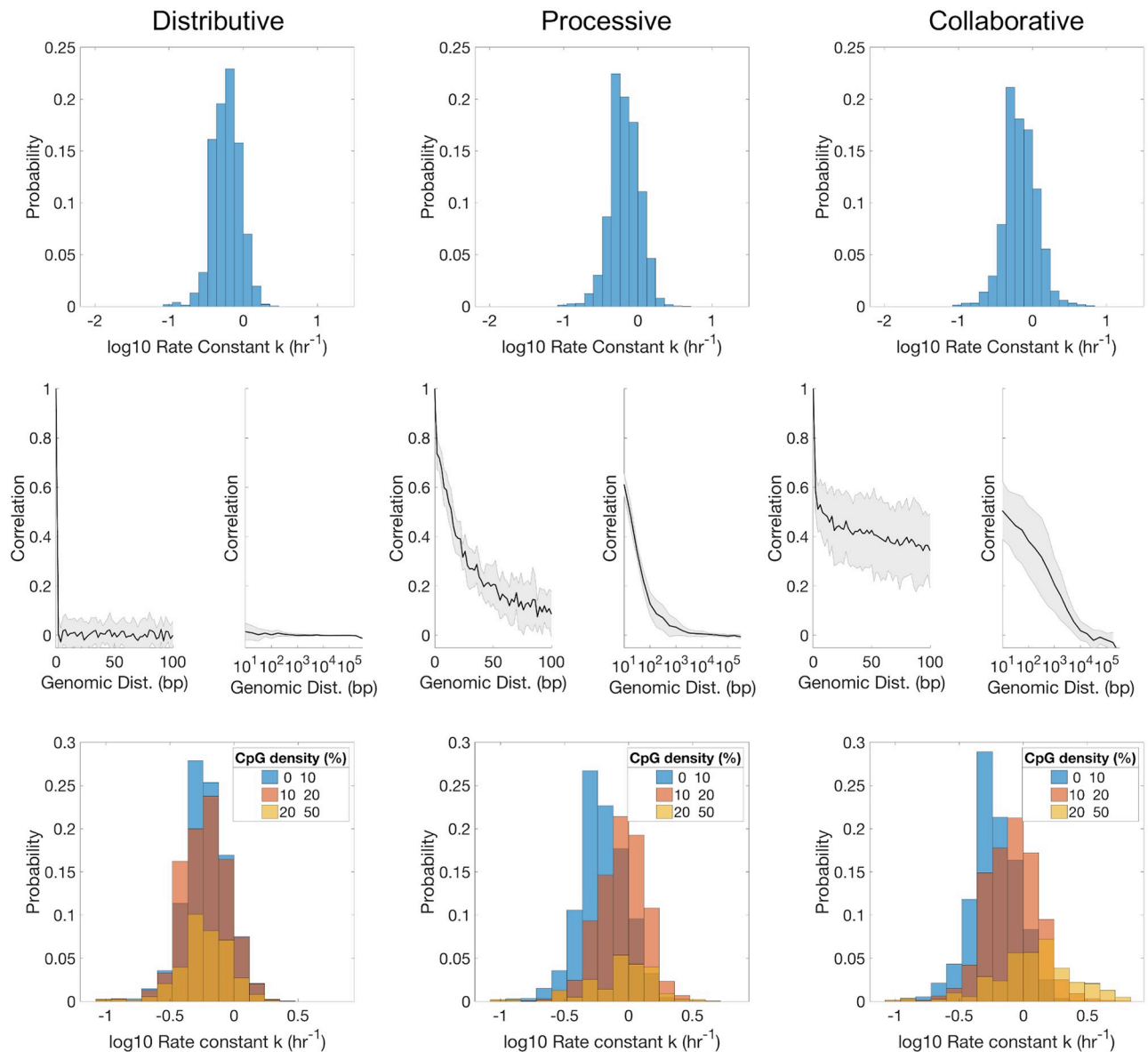
Fig 8. Simulated remethylation rate histograms (top), k -correlation with Genomic Distance (GD) (middle), and k -dependence on local CpG density ( CpG_d ) (bottom) when using each of the proposed mechanisms (Distributive, Processive, and Collaborative). The same in silico cluster containing 10^5 sites was used for all models. Both the position and the f_a for every site were sampled from an independent experimental dataset of WGBS measurements from Chr1 in arrested HUES64 cells [29].
