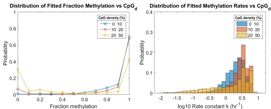
Fig 6. Remethylation rates and fraction methylation distributions for low, medium, and high-density CpG sites of Chr1. CpG density ( CpG_d ) of a site i is determined as the fraction of bp that are part of a CpG dinucleotide within a radius of 50 bp upstream and downstream the DNA molecule. Low-density CpG-sites represent 87% of the total sites analyzed in Chr1. Medium-density CpG sites represent a 12%, and high-density sites less than 1%. Low density is defined as [0,10)\% . Medium density is defined as [10,20)\% . High density is defined as [20, CpG_{d_{max}}]\% , where CpG_{d_{max}} is the maximum CpG_d found in Chr1 (50%).
