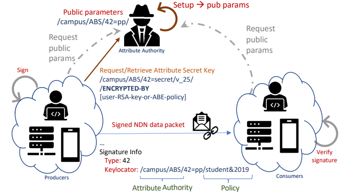
Figure 4: NDN-ABS naming and working
