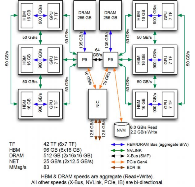
Figure 5: The architecture of a computational node on Summit.
