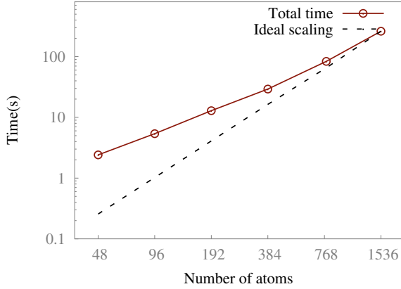
Figure 8: Weak scaling: wall clock time per 50 as for silicon systems with 48 to 1536 atoms. The number of GPUs used are always set to half of number of atoms in the calculation. The “ideal scaling” here scales as O(N_{\text{atom}}^2) .
