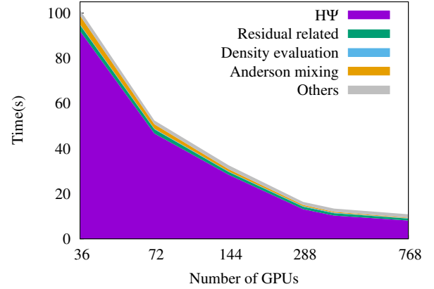
Figure 9: Strong scaling: the total time of a single SCF step and the contributions of each part using different number of GPUs.
