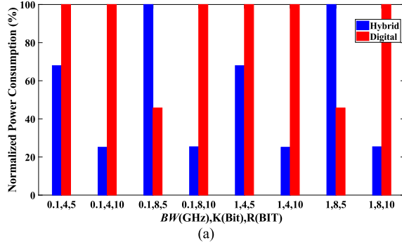
Fig. 10. Comparison of normalized power consumption against different combinations of bandwidth (BW), PI resolution (K), and ADC resolution (R) for (a) N = 16 , and (b) N = 128 , assuming power consumed in a 65 nm CMOS process for 8-bit PI as 44 mW/200 MHz, 5-bit OTA as 3 mW/4 Inputs/100 MHz, and 5-bit ADC (described in [26]) as 1.2 mW/250 MHz.
