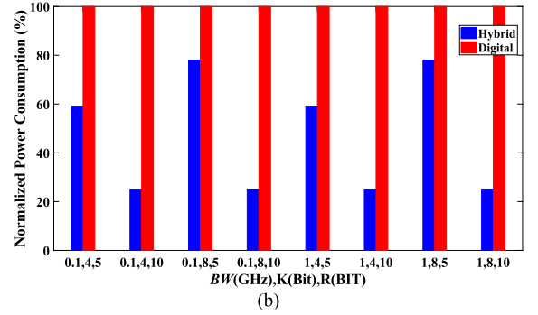
Fig. 10. Comparison of normalized power consumption against different combinations of bandwidth (BW), PI resolution (K), and ADC resolution (R) for (a) N = 16 , and (b) N = 128 , assuming power consumed in a 65 nm CMOS process for 8-bit PI as 44 mW/200 MHz, 5-bit OTA as 3 mW/4 Inputs/100 MHz, and 5-bit ADC (described in [26]) as 1.2 mW/250 MHz.
