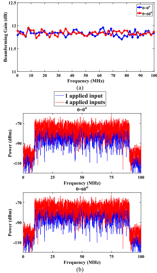
Fig. 11. Simulation results for: (a) beamforming gain for a single-tone signal for two different AoAs, and (b) 80 MHz BW signal for two different AoAs.
