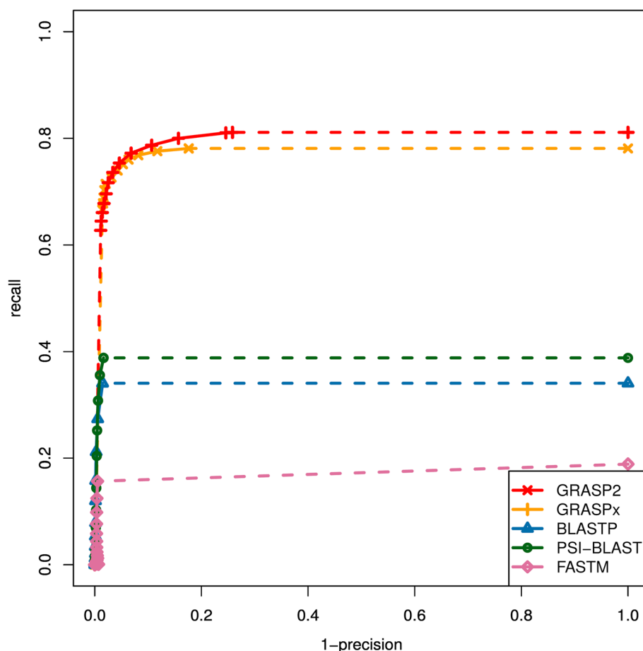
Fig. 2 The Receiver Operating Characteristic (ROC) curves for the performances of GRASP2, GRASPx, BLASTP, PSI-BLAST, and FASTM on the marker gene reference set. GRASP2 and GRASPx have the highest performance among all programs that have been benchmarked. The dotted lines correspond to extrapolated performances
