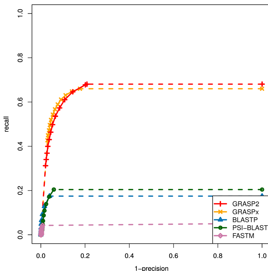
Fig. 3 The Receiver Operating Characteristic (ROC) curves for the performances of GRASP2, GRASPx, BLASTP, PSI-BLAST, and FASTM on the whole genome reference set. GRASP2 and GRASPx have the highest performance among all programs that have been benchmarked. The dotted lines correspond to extrapolated performances
