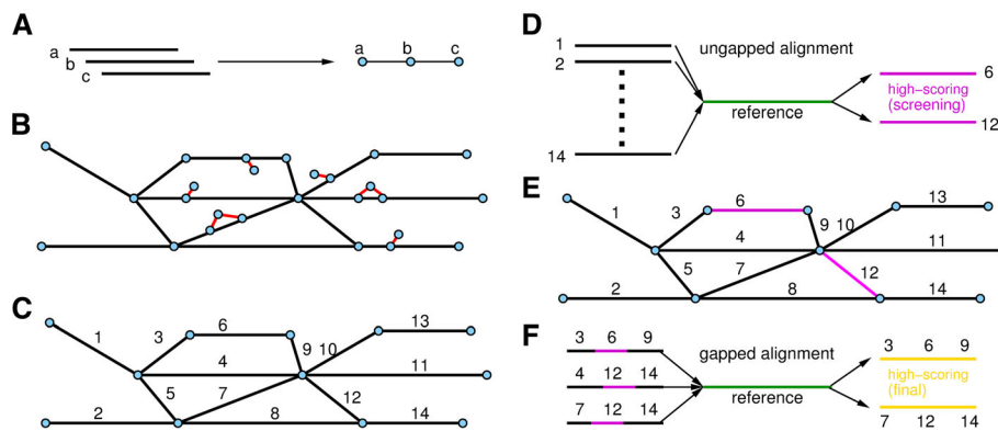
Fig. 1 Overview of the GRASP2 algorithm. a The reads are overlapped to construct an assembly string graph. b Bubbles and tips are identified and subsequently removed from the assembly graph. c Unbranched paths are collapsed into single edges. Each collapsed edge is considered as a unitig and receives an arbitrary label. d Ungapped alignment is performed between the reference protein sequence and each of the unitig. e High-scoring unitigs are treated as anchors to initialize gapped alignments. f Candidate paths are generated based on the identified anchor unitigs. Gapped alignment is performed between the reference protein sequence against the candidate paths to recruit homologous paths
