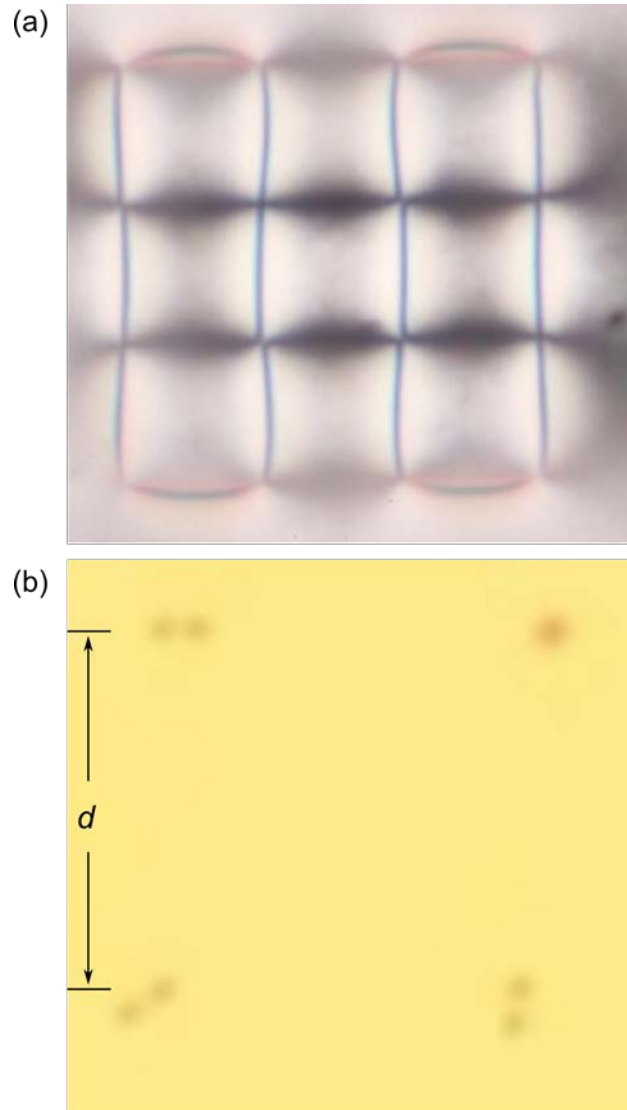
FIG. 1. Nematic LC cell with line defects. a) Experimental polarising microscopy texture of a nematic LC cell exhibiting line defects confined near the master plate. b) Bright field image of a section of the sample showing three of the four integer s=\pm 1 defects having decomposed into half-integer defects.
