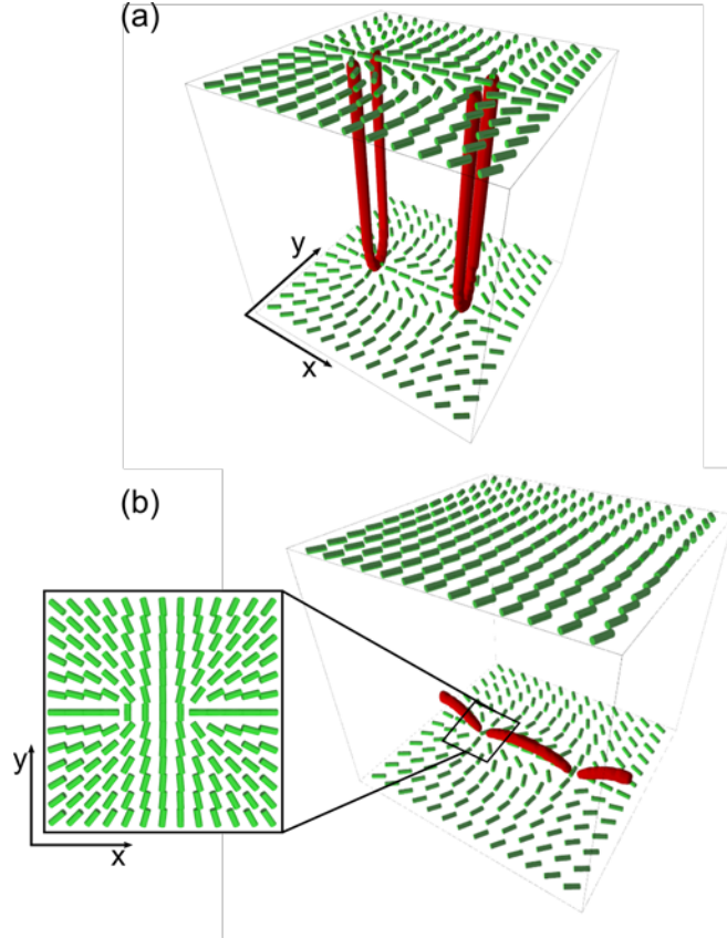
FIG. 4. Schematic sketches showing cells possessing either charged or chargeless line defects, where the master plate enforces s=\pm 1 surface point defects. a) Charged s=1/2 split disclination lines spanning the master and slave confining plate. b) Chargeless line defects joining s=\pm 1/2 daughter defects within the master plate. Typical director field profiles are shown both just above the master plate and well above it. The red line indicates region where the amplitude S = \sqrt{\frac{3}{2} \text{Tr} \mathbf{Q}^2} of the order parameter \mathbf{Q} is reduced to S = S_{\text{bulk}}/2 due to strong local elastic distortions. Here S_{\text{bulk}} stands for the bulk equilibrium value.
