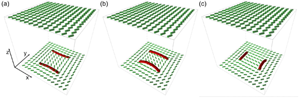
FIG. 9. Different stages of the thickness-driven rewiring mechanism shown for the case of a 2 \times 2 array of s=\pm 1/2 master plate imposed surface defects. a) \frac{d_y}{d_x} = 1 , b) \frac{d_y}{d_x} = \frac{4}{5} , c) \frac{d_y}{d_x} = \frac{3}{5} . The nematic director field is plotted just above the master plate and at the slave plate, and we superimpose the line defect profile. (Points are plotted where the order parameter is strongly suppressed due to elastic distortions). Scale bar corresponds to the cell thickness h .
