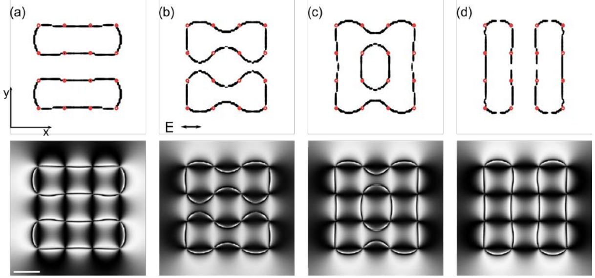
FIG. 10. Numerical simulation of the external electric field driven rewiring shown for the case of a 4 \times 4 array of s=\pm 1 master plate imposed surface defects. Selected stages of the transition between two different realizations of structure depicted in Fig. 5a are shown. The top rows: The top cell view of the line defect patterns where regions with strongly suppressed order parameter values are shown. The bottom row: The corresponding calculated optical microscopy textures obtained under crossed polarizers. All structures and interference patterns were obtained numerically. In the simulation we gradually increase E . a) \xi_b/\xi_E = 0 , b) \xi_b/\xi_E = 1.12 , c) \xi_b/\xi_E = 1.23 , d) \xi_b/\xi_E = 1.34 . Scale bar corresponds to the cell thickness h .
