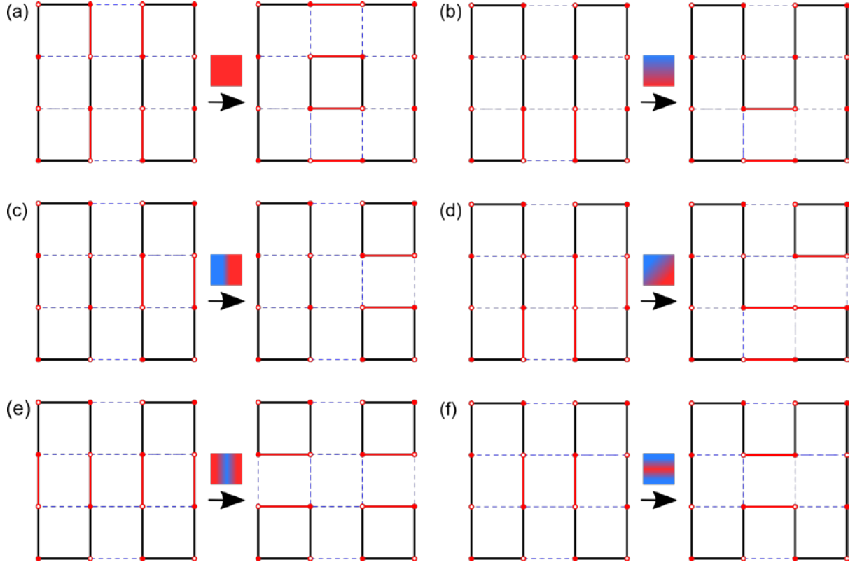
FIG. 7. Schematic representation of rewiring between different irreducible patterns. a) [II] \rightarrow [O] , b) [II] \rightarrow [U] , c) [II] \rightarrow [loo] , d) [II] \rightarrow [Lo] , e) [II] \rightarrow [oooo] , f) [II] \rightarrow [H] . Disclinations marked in red are rewired in the transformation. This may be accomplished, for example, by using a spatially-dependent electric field: In the coloured squares above the arrows we schematically indicate the external electric field \mathbf{E} spatial profile. Red and blue colour mark a relatively large and zero value of E , respectively. The diffuse regions correspond to spatially slow variation of field \mathbf{E} ; the sharp transitions between red and blue correspond to a spatially rapid variation of \mathbf{E} . Note that for all cases only the pairs of facing disclinations need to be rewired.
