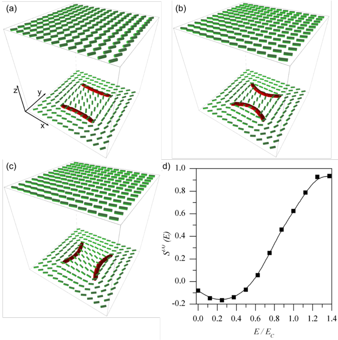
FIG. 8. Different stages of the electrical field-driven rewiring mechanism shown for the case of a 2 \times 2 array of s=\pm 1/2 master plate imposed defects. a) E=0 , b) E \lesssim E_c ( \xi_E = 1.118 \xi_b ), c) E \gtrsim E_c ( \xi_E = 0.994 \xi_b ). At E = E_c (corresponding to \xi_E \sim \xi_b ) the defect lines rewire. The nematic director field is plotted just above the master plate and at the slave plate, and we superimpose the line defect profile. (Points are plotted where the order parameter is strongly suppressed due to elastic distortions). d) S^{(x)}(E) vs. E/E_c is plotted. Calculated points are marked by square symbols and the line is the guide for an eye. Scale bar corresponds to the cell thickness h .
